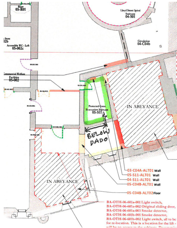
Alterations Plan 05 - 01 SOUTH WEST 1:100
