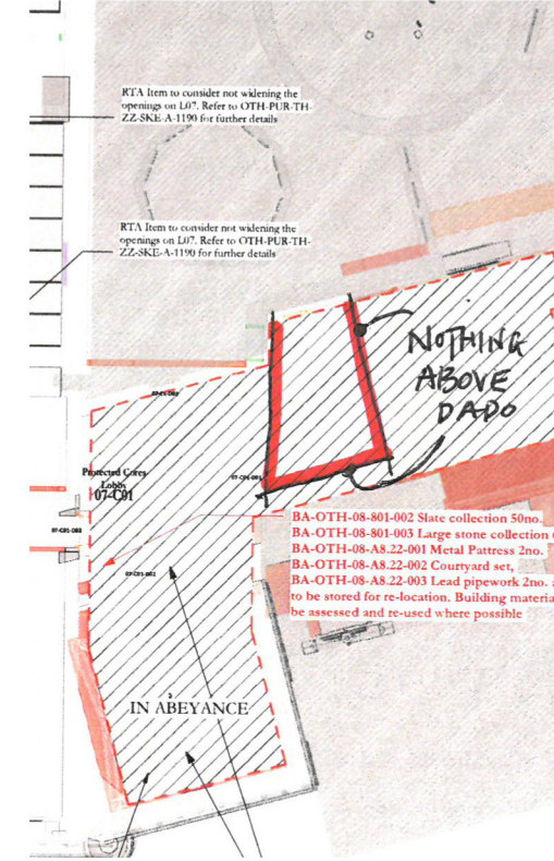
Alteration Plan 07 - 01 SOUTH-WEST 1:100
