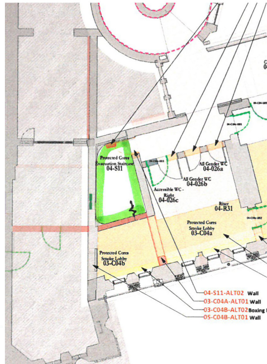
Alteration Plan 04 - 01 SOUTH-WEST 1:100
