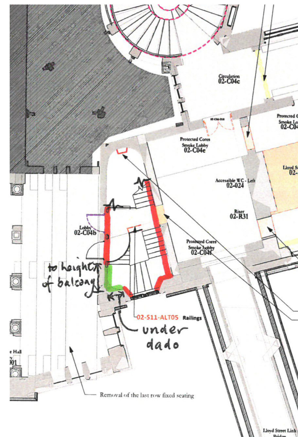
Alterations Plan 02 - 01 SOUTH WEST 1:100
