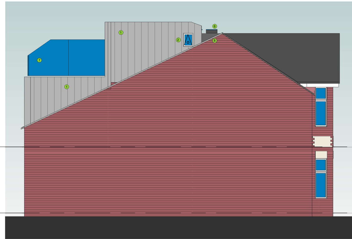
2 West Elevation Proposed 1 : 100
