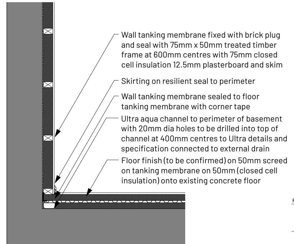
4 Typical Existing External Wall Detail Scale: 1:20
