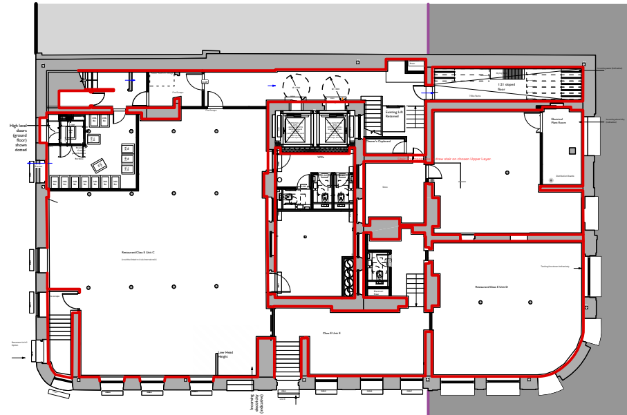
1 Perimeter Drain Basement Plan Scale: 1:300
