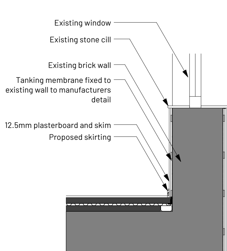
2 Existing Window Tanking Detail Scale: 1:20
