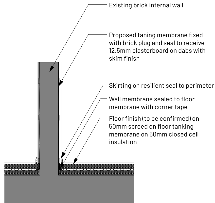
3 Existing Internal Wall Tanking Detail Scale: 1:20
