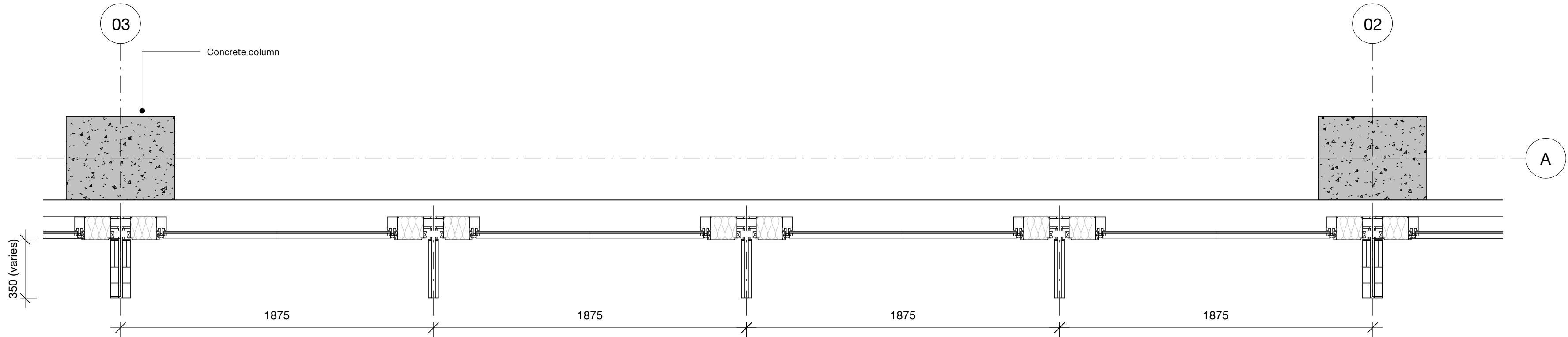
02 Typical Bay Elevation 21001 1 : 20
