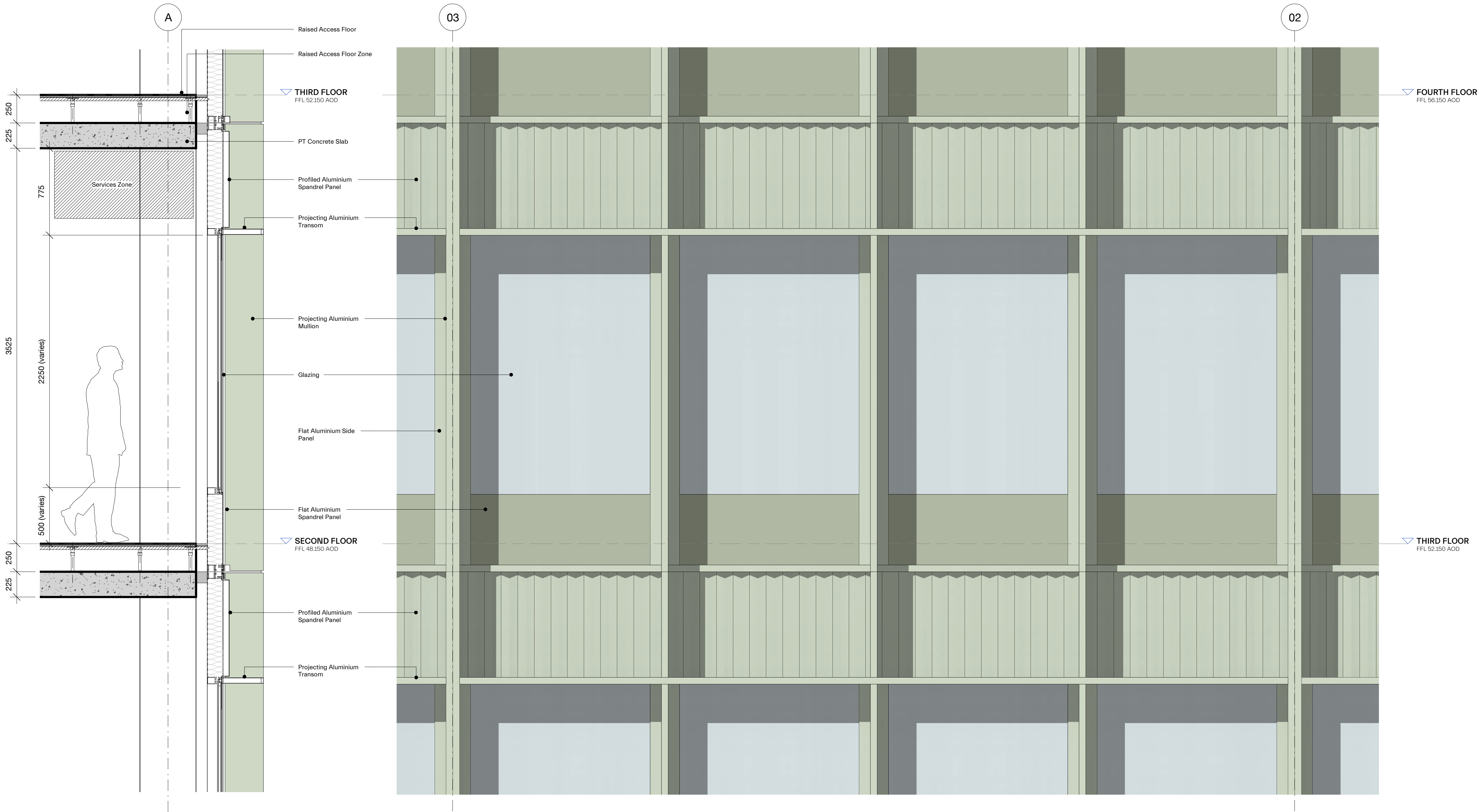
03 Typical Bay Section 21001 1 : 20
