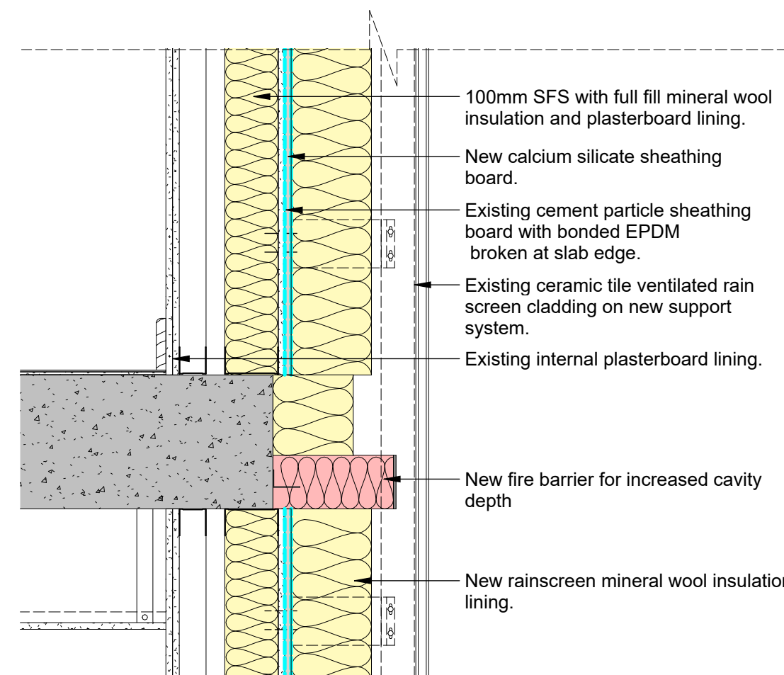
S2 Proposed Typical Terracotta Rainscreen Detail 1:10
