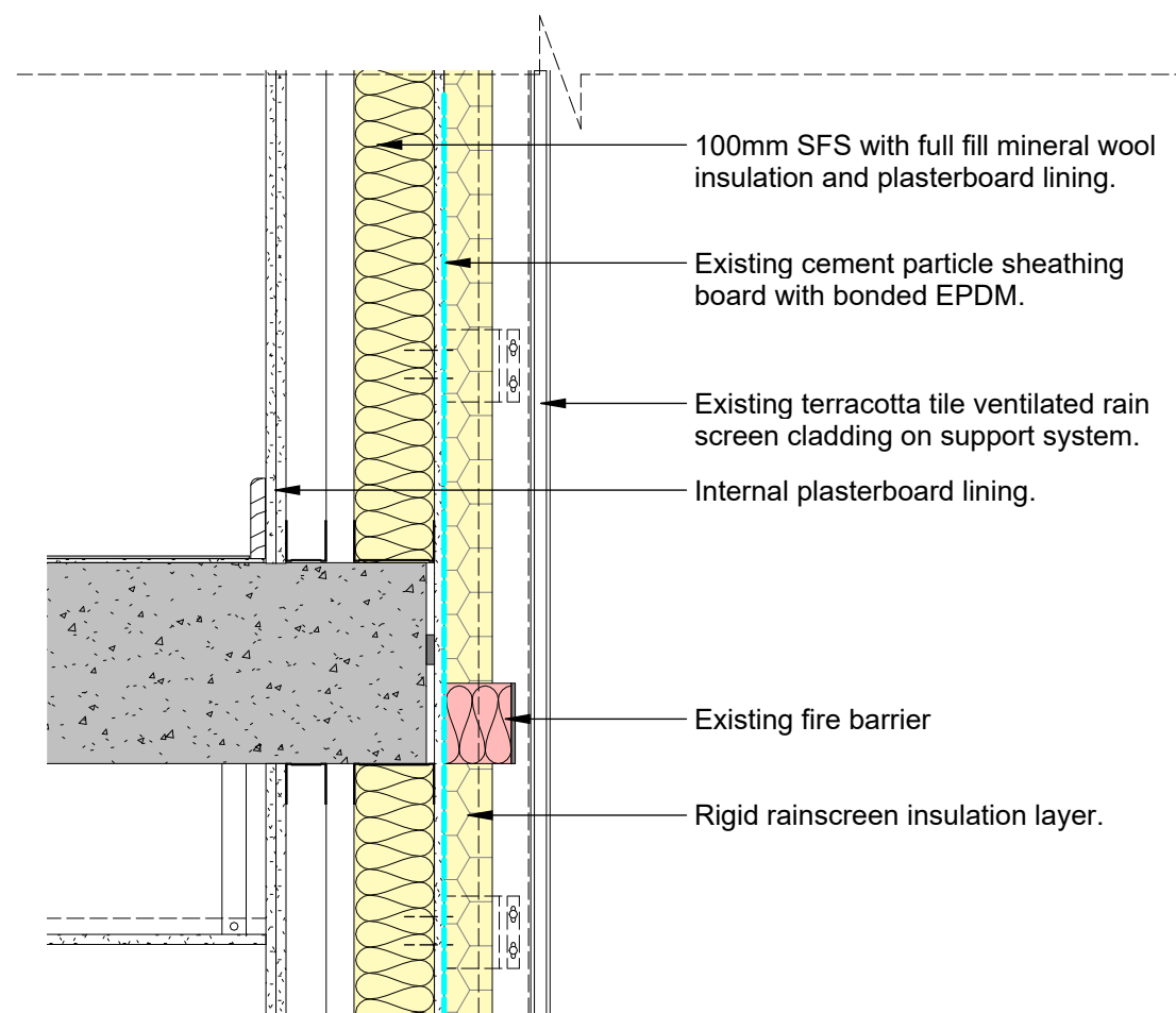
S1 Existing Typical Terracotta Rainscreen Detail 1:10
