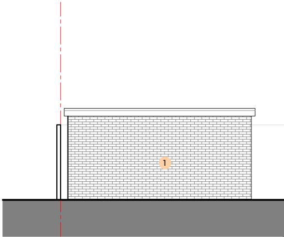
OUTBUILDING PROPOSED LEFT SIDE ELEVATION 1:100 @ A3
