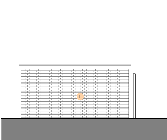
OUTBUILDING PROPOSED RIGHT SIDE ELEVATION 1:100 @ A3
