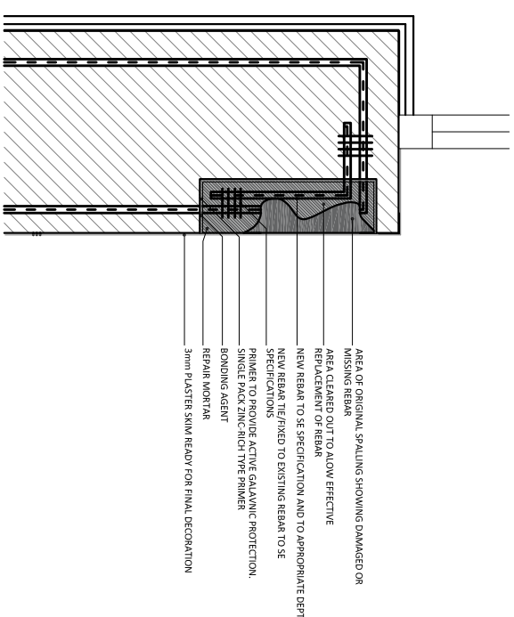
TYPICAL SPALLED CONCRETE WITH DAMAGED REBAR REPAIR 1:10
