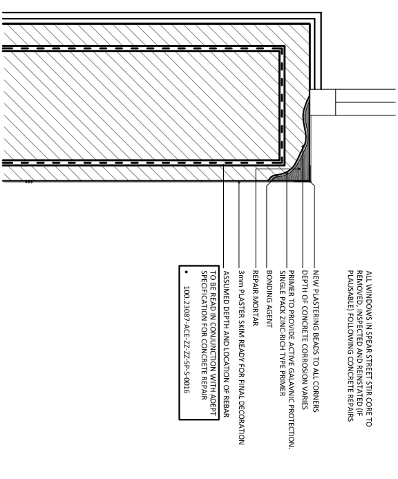
TYPICAL SPALLED CONCRETE CILL/JAMB/HEAD REPAIR 1:10
