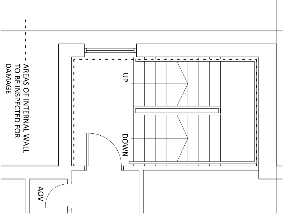
DAMAGED AREAS FOR INSPECTION 1:50
