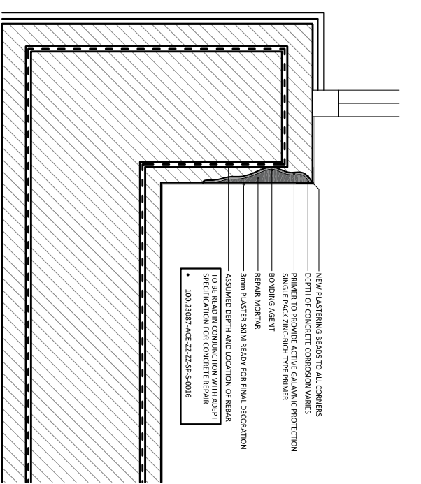
TYPICAL SPALLED CONCRETE REPAIR 1:10
