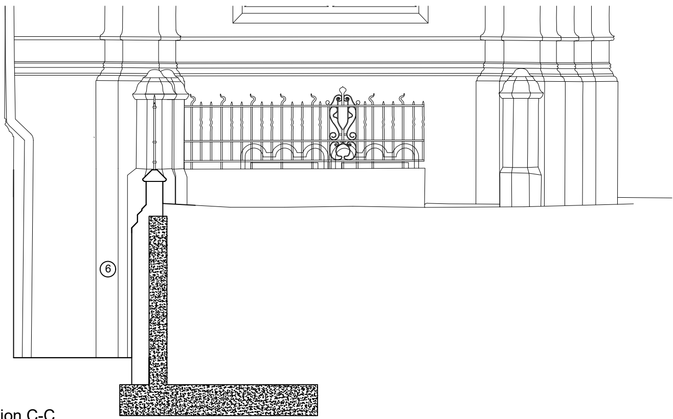
Section C-C
