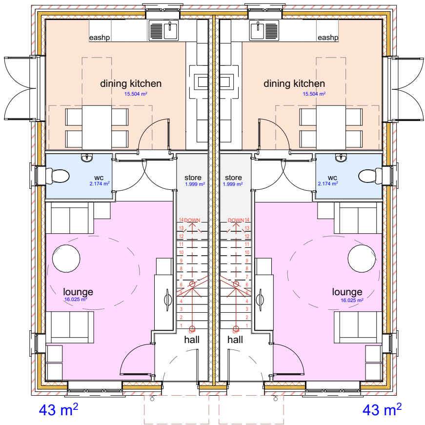
1 GF-Ground Floor 1:100
