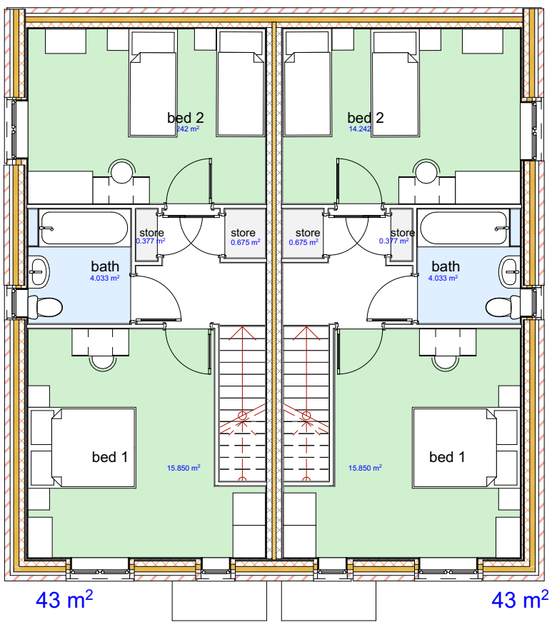
2 01-First Floor 1:100
