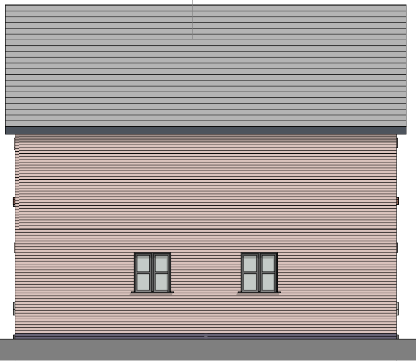
Rear Elevation 1:100
