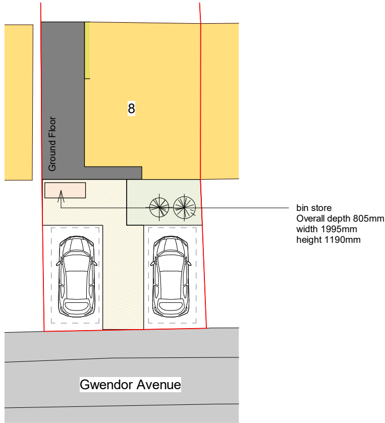
3. Site Location Plan - Proposed Bin Store 1 : 200
