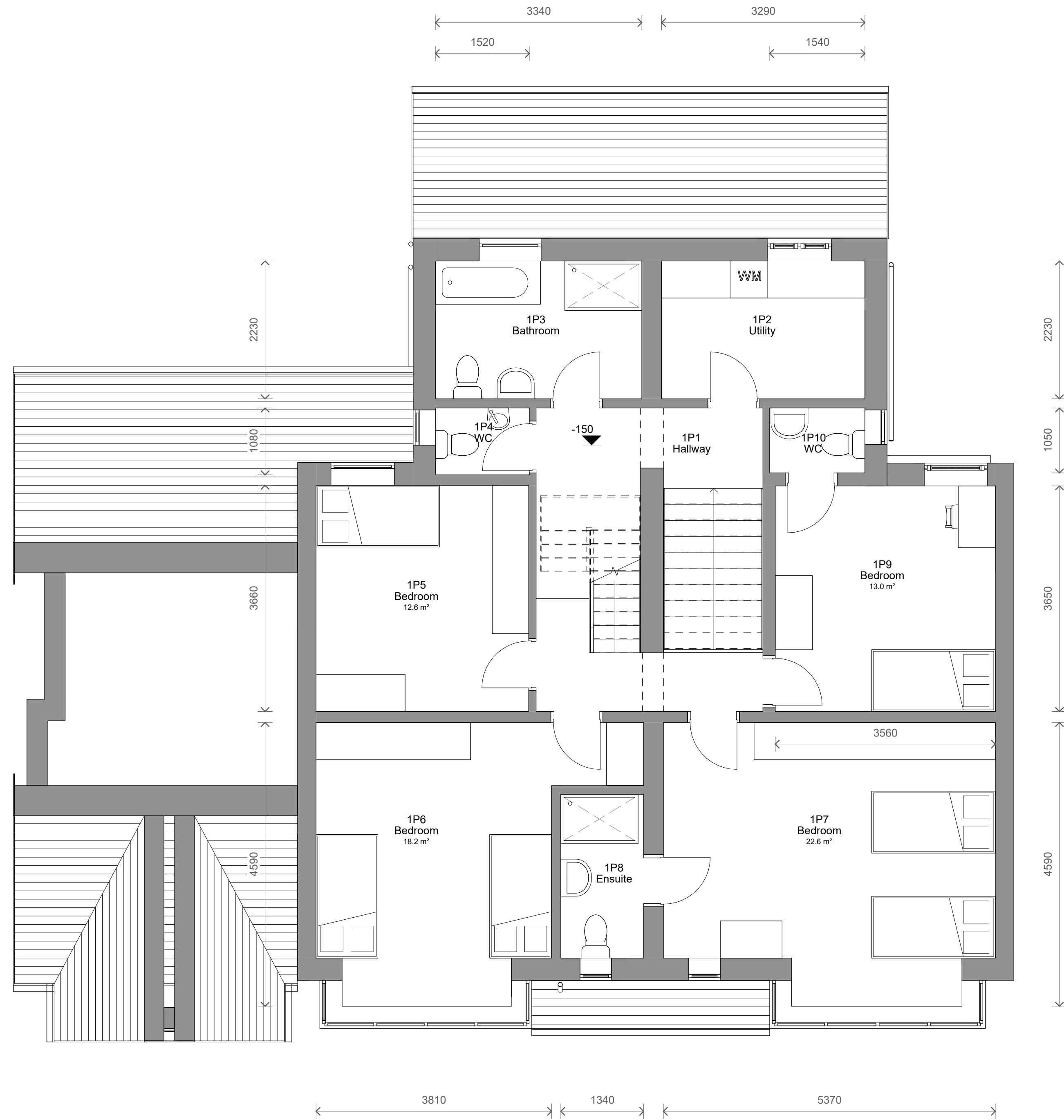
2 Level 1 - Proposed 1 : 50
