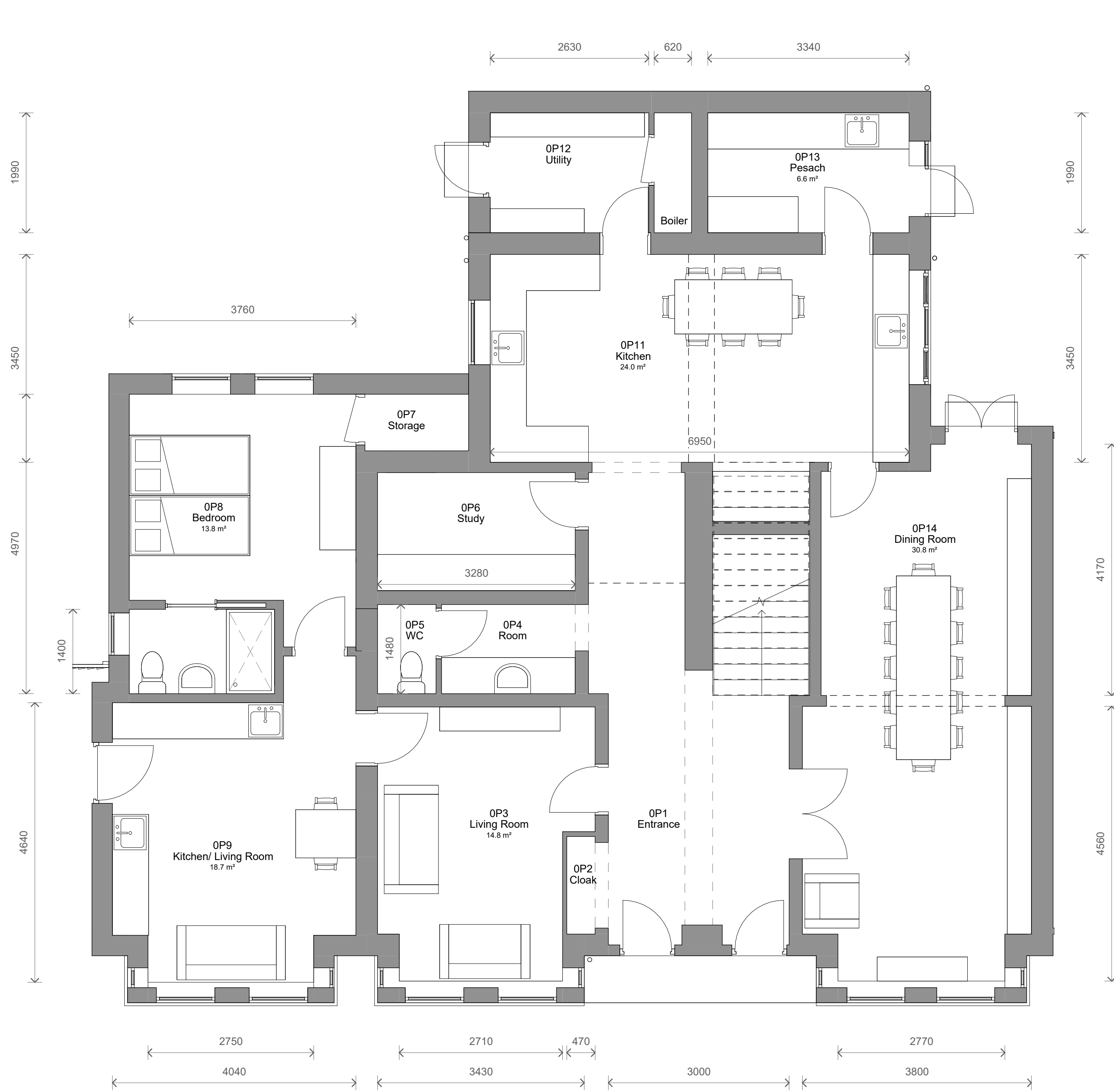
1 Level 0 - Proposed 1 : 50
