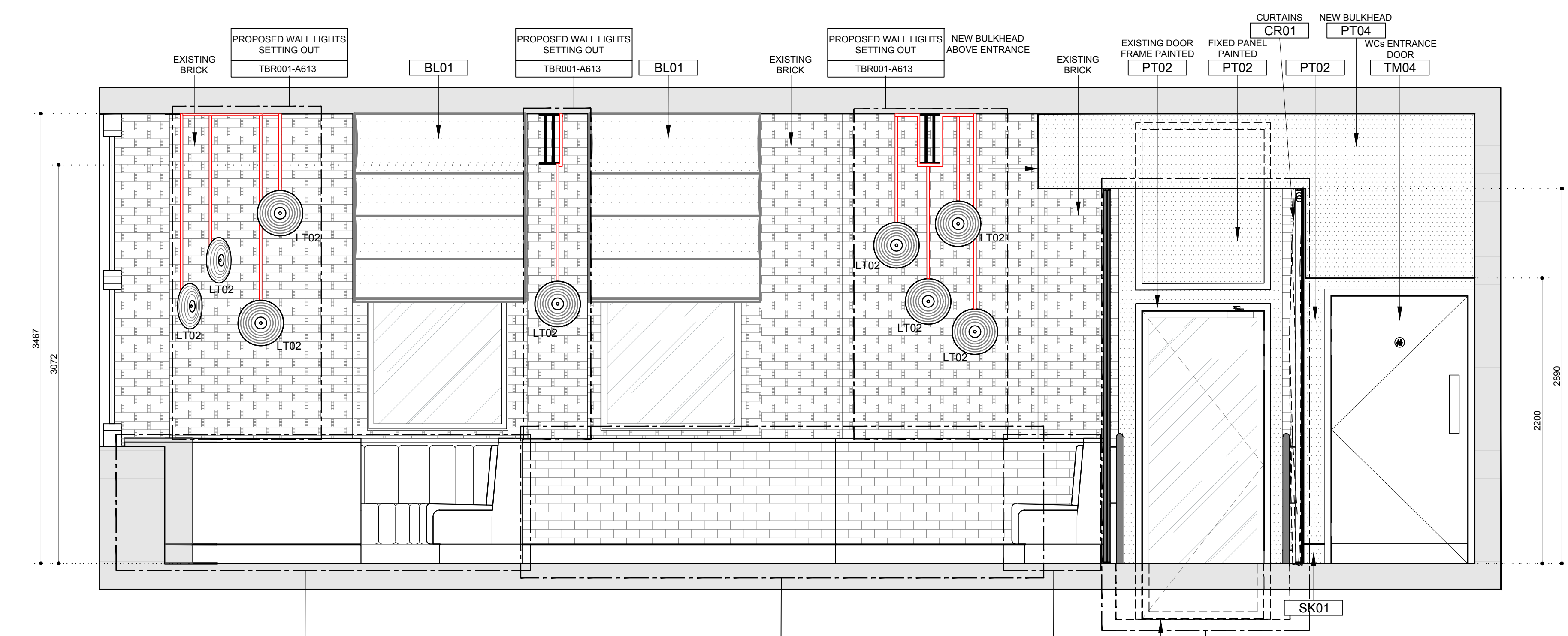
02 ELEVATION B SCALE 1:25 @ A1 PROPOSED BOOTH DETAILS TBR001-A611 PROPOSED TILE & TIMBER CLADDING DETAILS TBR001-A612 PROPOSED BANQUETTE DETAILS TBR001-A609 PROPOSED ENTRANCE RAMP DETAILS TBR001-A600
