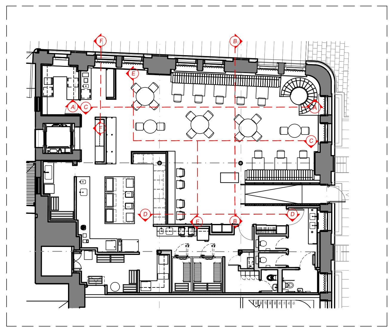
00 KEY PLAN SCALE 1:150 @ A1
