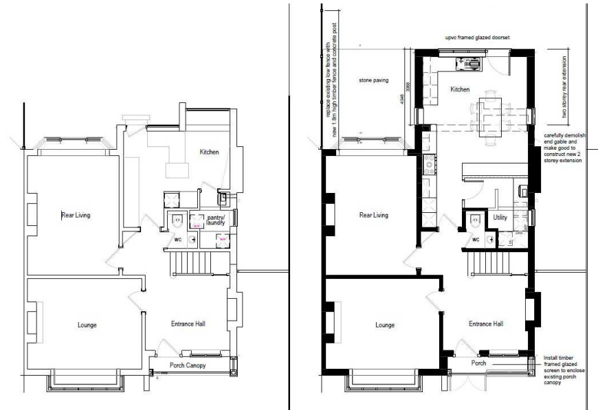
Fig.09 Existing Ground Floor (above) & Proposed Ground Floor (RHS)
