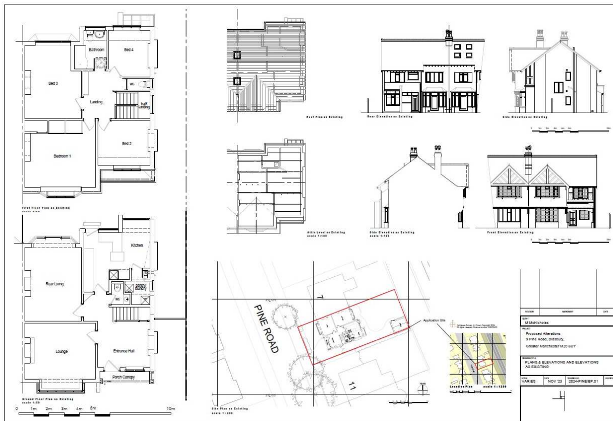
Fig. 07 Existing Plans and Elevations
