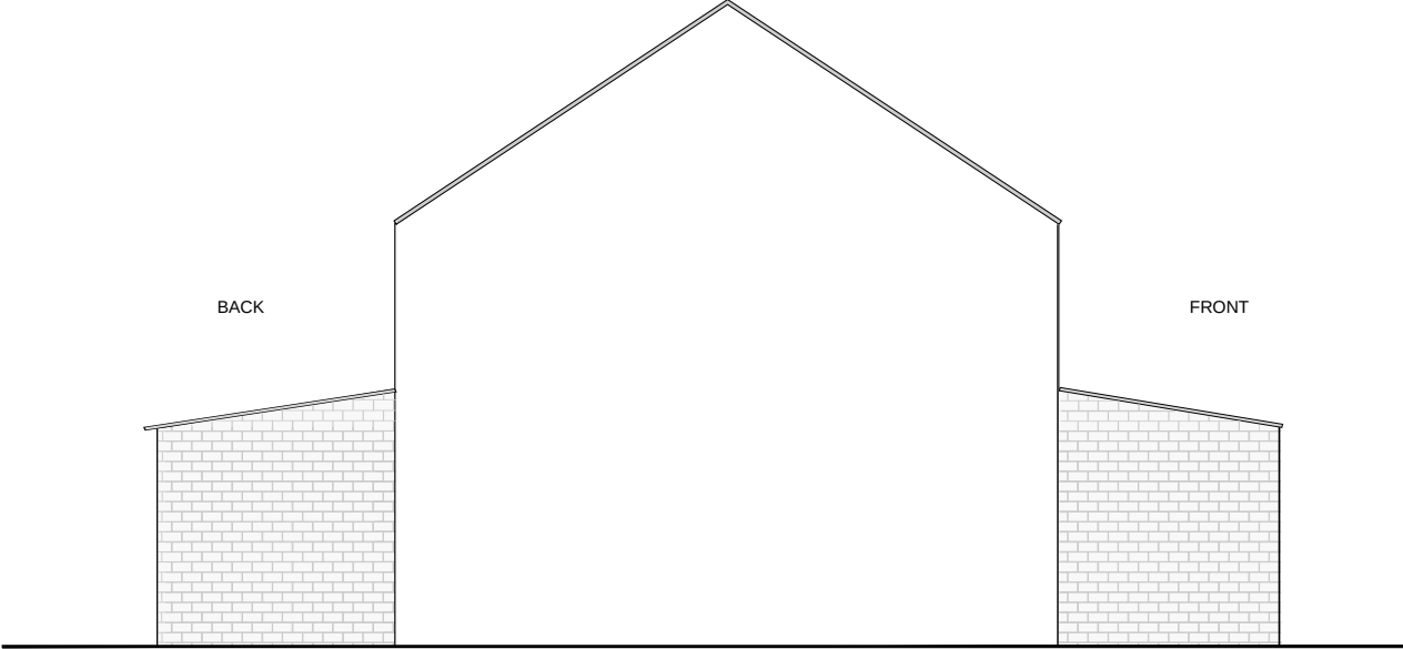
THE ADJOINING PROPERTY PROPOSED SIDE ELEVATION VIEW
