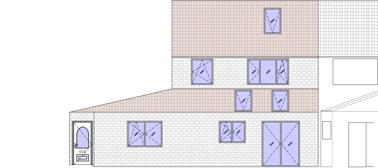
BACK ELEVATION
