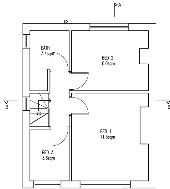
EXISTING FIRST FLOOR PLAN 1:100 @ A3
