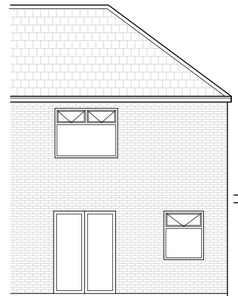
EXISTING FRONT ELEVATION 1:100 @ A3
