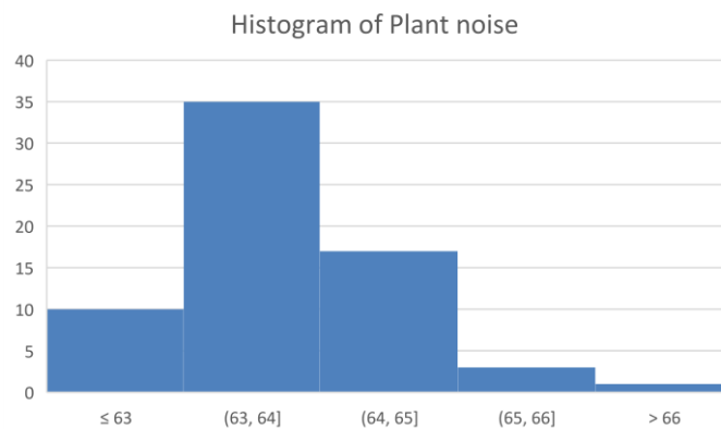
Figure 7 Histogram of plant noise
