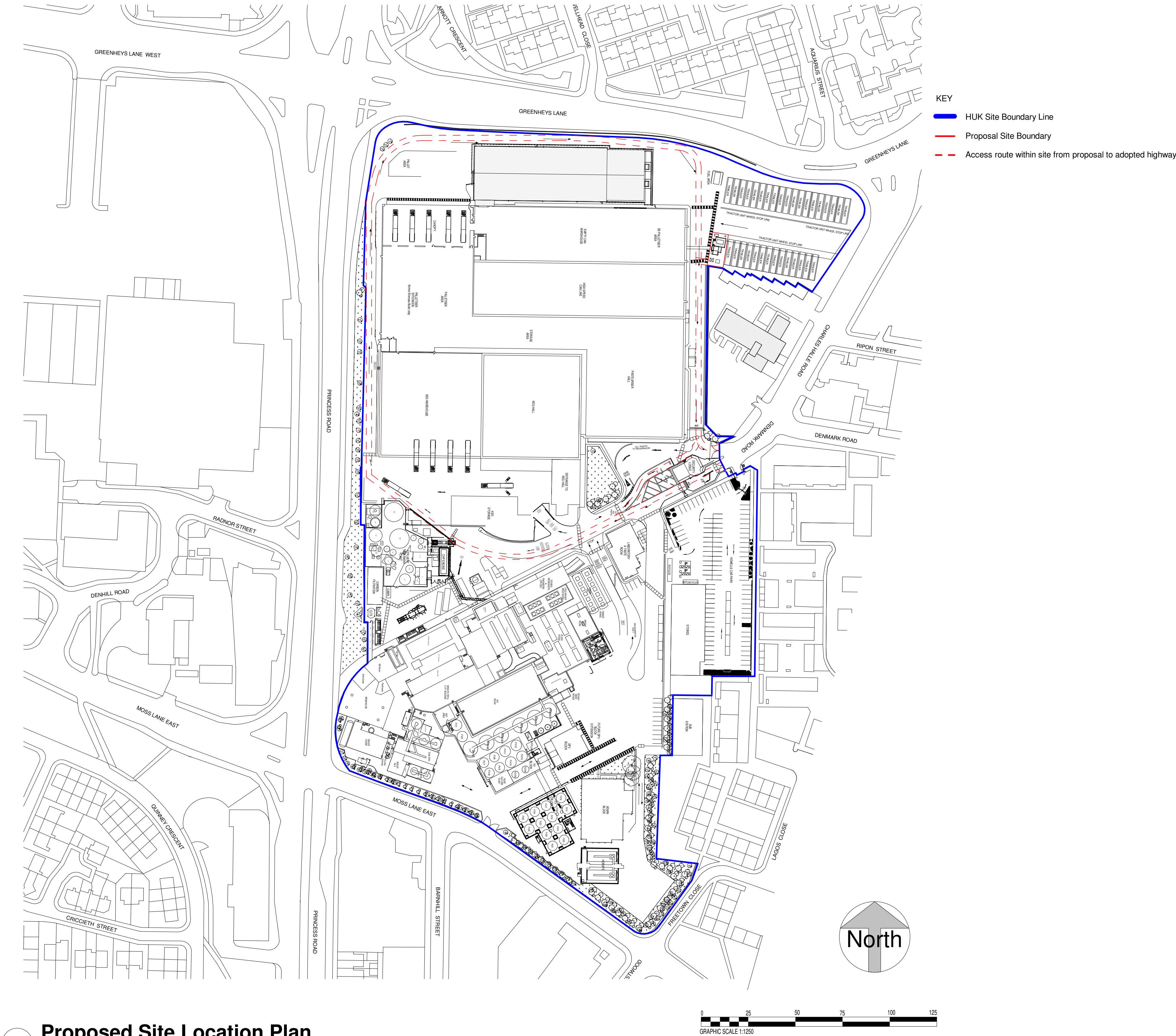
1 Proposed Site Location Plan 1 : 1250
