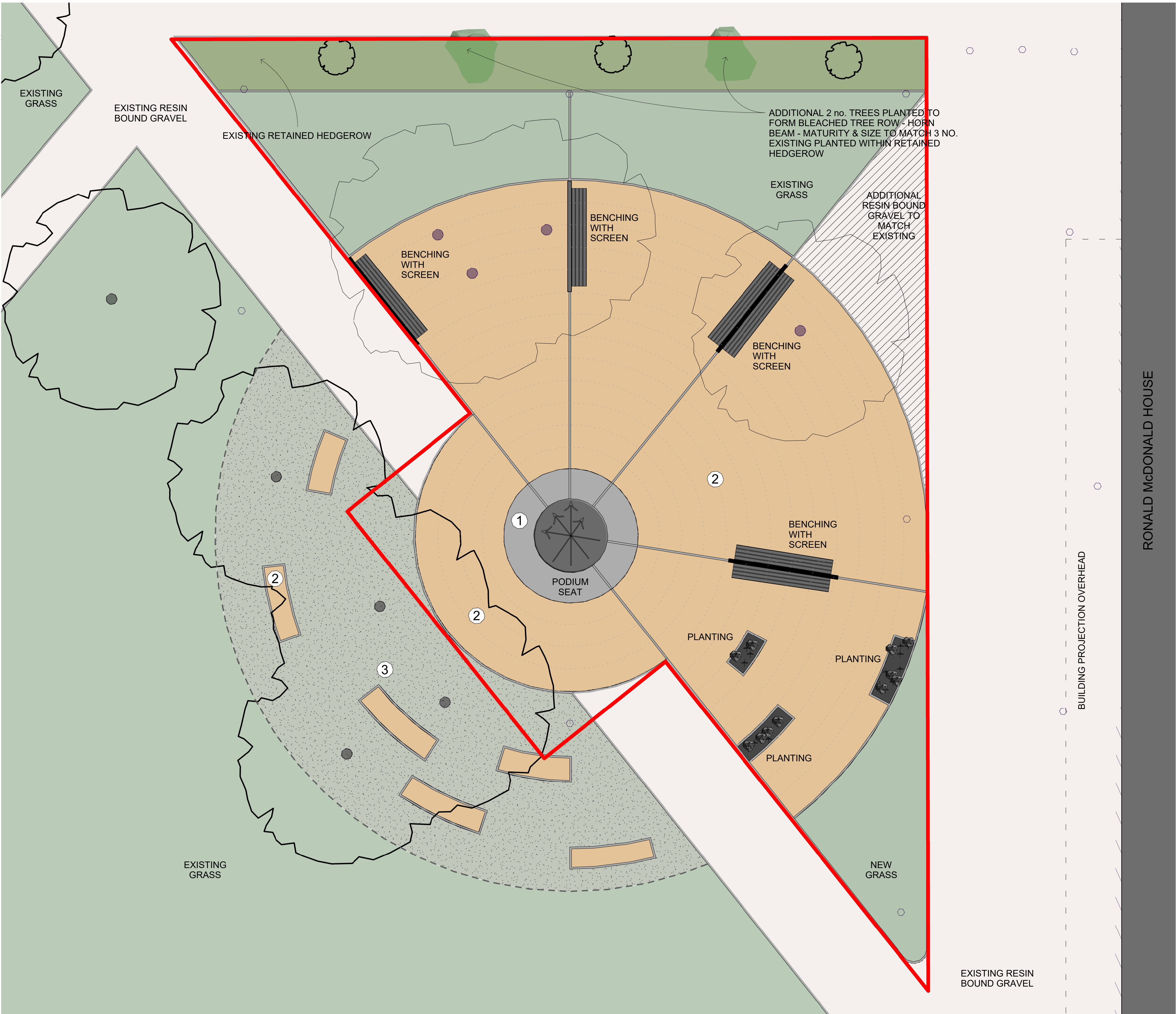
1 Proposed Site Plan 1:50
