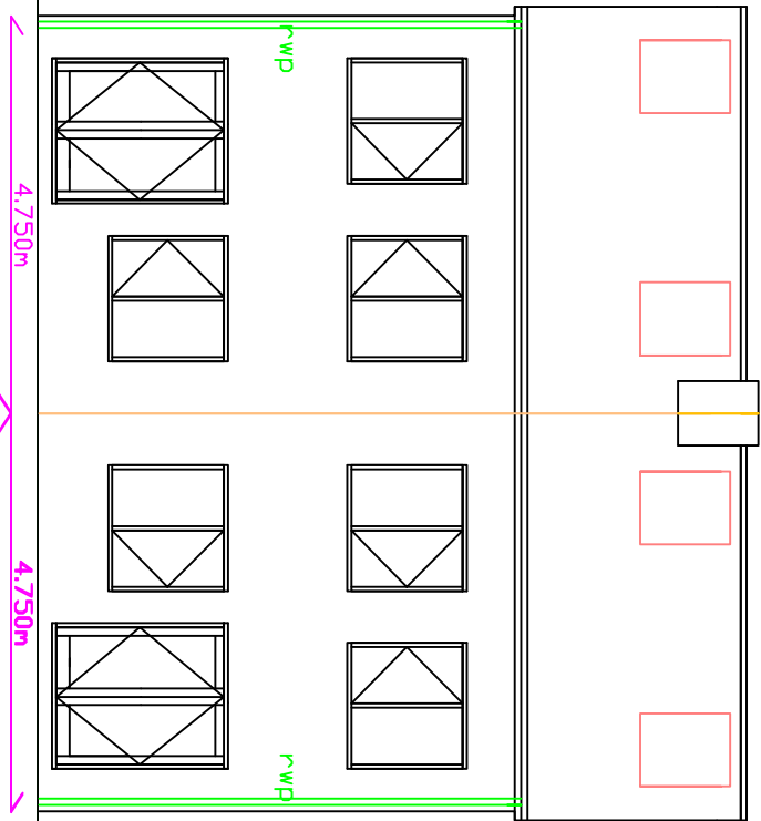
PROPOSED REAR WEST VIEW PLOT A&B 1: 100
