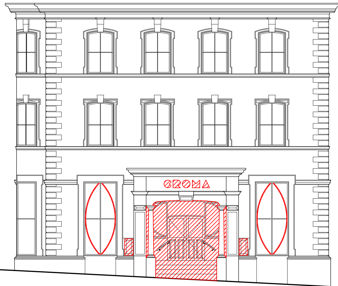
EXISTING NORTHWEST ELEVATION CLARENCE STREET FACADE DEMOLITIONS SHOWN IN RED
