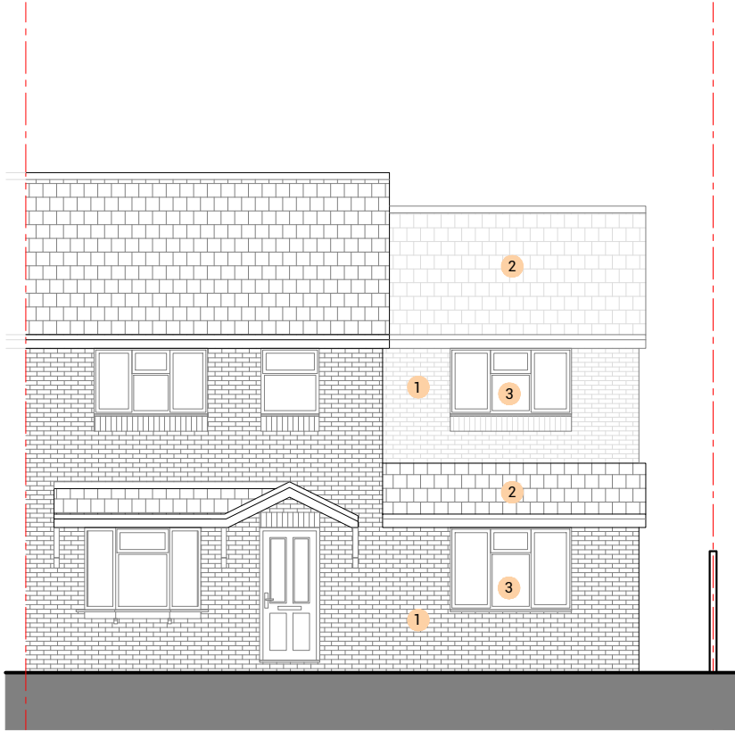
PROPOSED FRONT ELEVATION 1:100 @ A3 0m 1m 3m 5m Key 1 Brickwork to match existing 2 Roof tiles to match existing 3 PVC Window to match existing 4 PVC Window to match existing (Obscure Glazing) 5 Glazed Bifold Door 6 Rooflight
