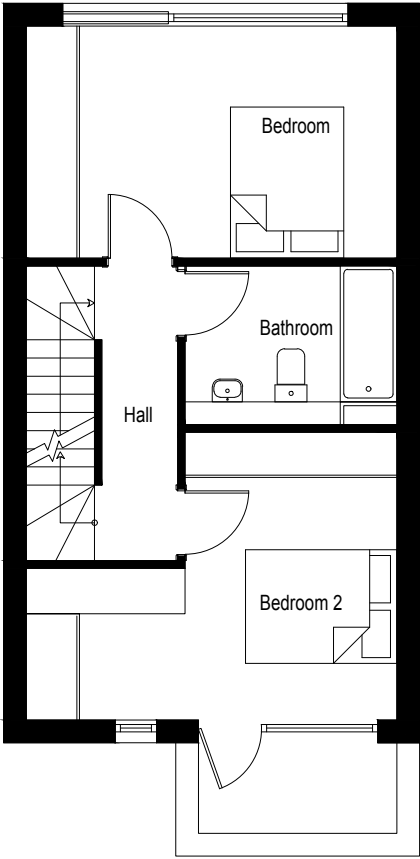
Proposed Type 01 GA First Floor Plan
