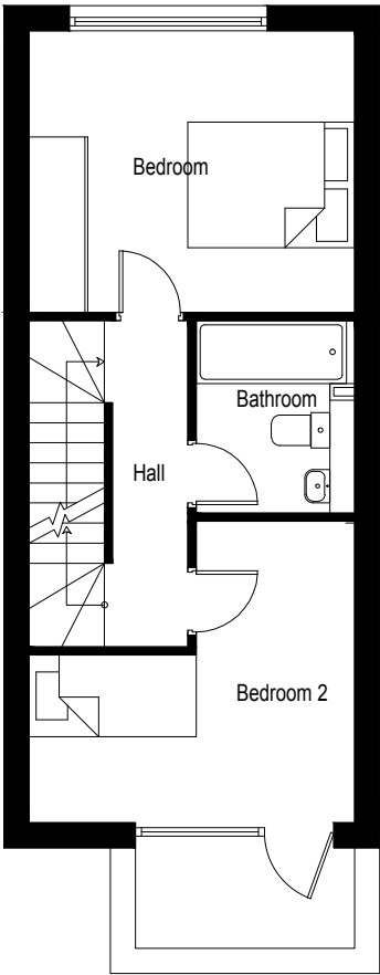
Proposed Type 02 GA First Floor Plan
