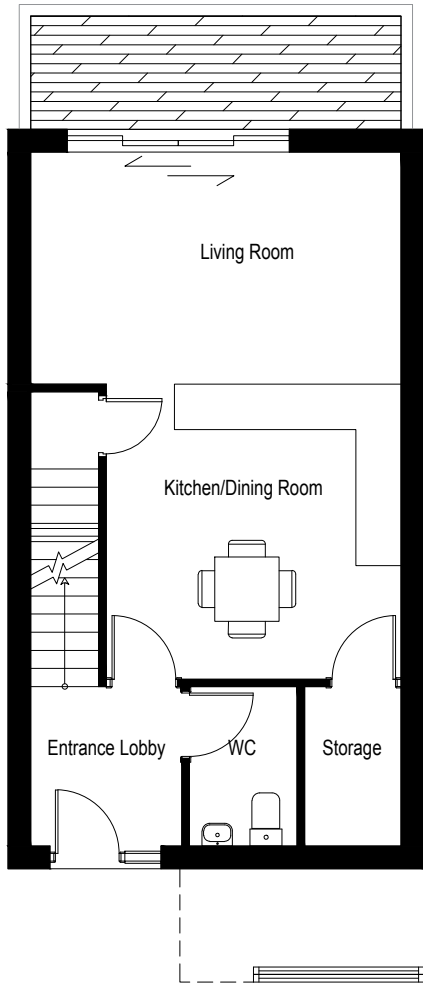
Proposed Type 01 GA Ground Floor Plan
