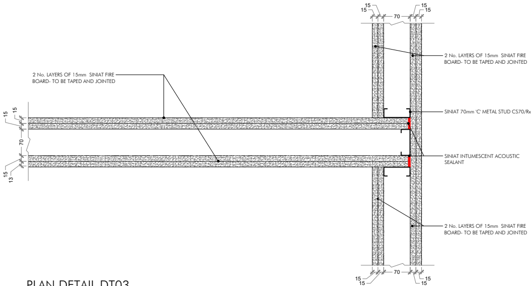
PLAN DETAIL DT03 TYPICAL PARTITION 'TYPE E' T JUNCTION SINIAT REFERENCE CS70R-215F SCALE 1:5
