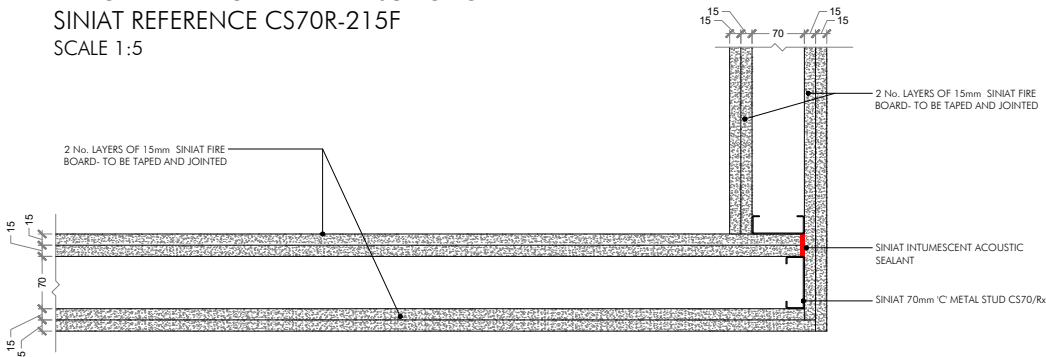
PLAN DETAIL DT04 TYPICAL PARTITION 'TYPE E' 90 DEGREE CORNER SINIAT REFERENCE CS70R-215F SCALE 1:5
