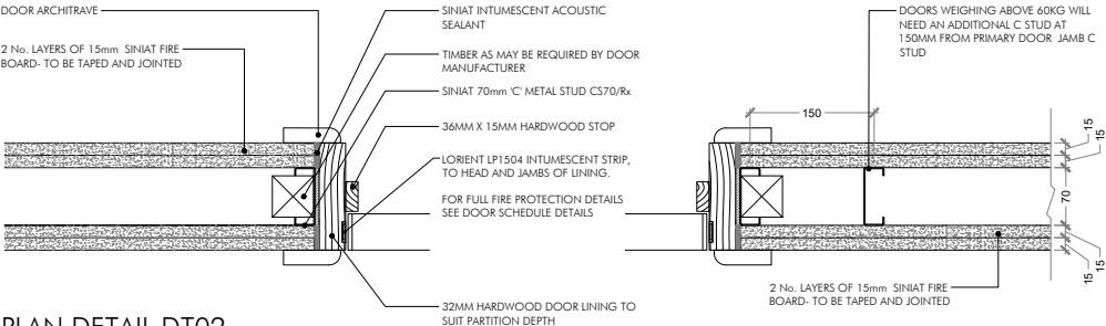
PLAN DETAIL DT02 TYPICAL PARTITION 'TYPE E' DOOR JAMB DETAIL (60 MIN FIRE RATED DOOR) SINIAT REFERENCE CS70R-215F SCALE 1:5
