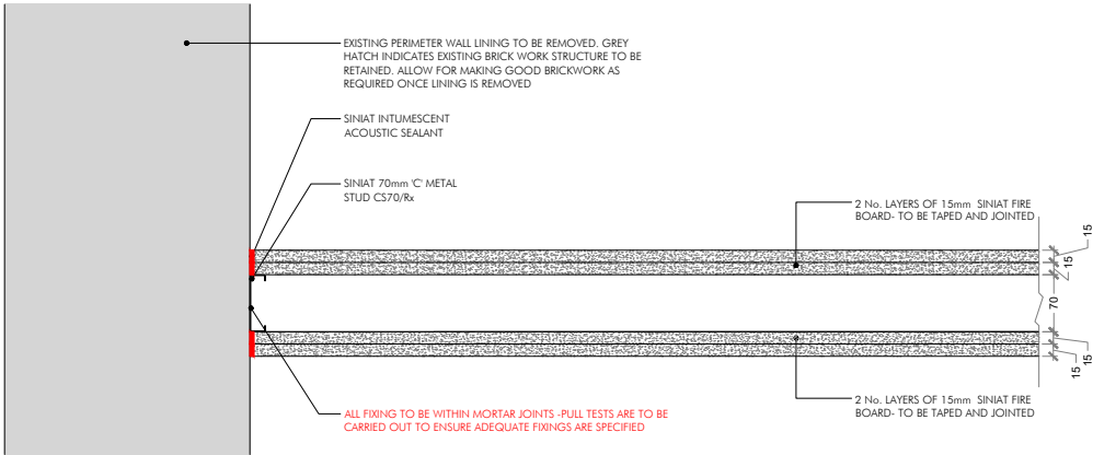
PLAN DETAIL DT01 TYPICAL PARTITION 'TYPE E' ABUTMENT WITH EXISTING WALL SINIAT REFERENCE CS70R-215F SCALE 1:5
