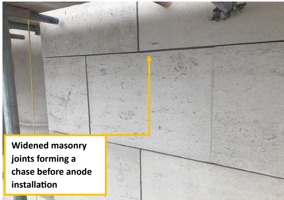
Widened masonry joints forming a chase before anode installation
