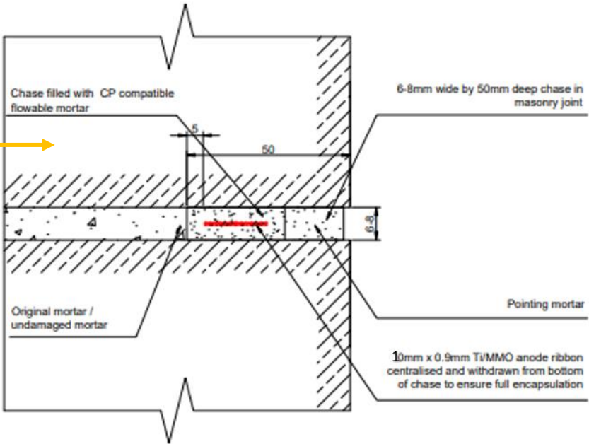
DETAIL 1 - RIBBON ANODE INSTALLATION SCALE 1:1 @ A1
