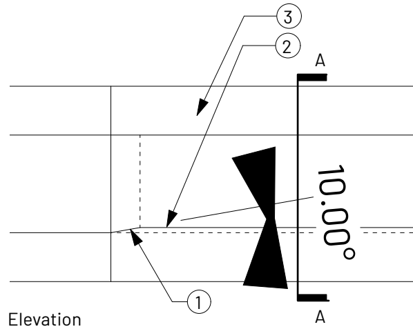
3 Localised Details - Cantilevered Stone Scale: 1:10
