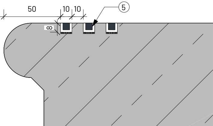
2 Localised Details - Stair Inserts Scale: Half Actual Size
