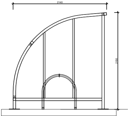
Cycle Store Side Elevation 6m Wardale Cycle Store (14 cycle capacity) 1:50@A3
