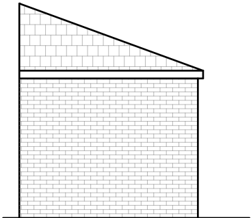
PREVIOUS SIDE ELEVATION
