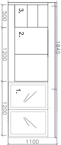
South Elevation scale 1/50
