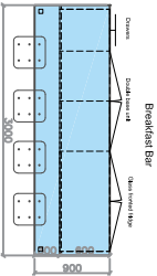
J05. Tea Point Suite 1. Scale 1/100
