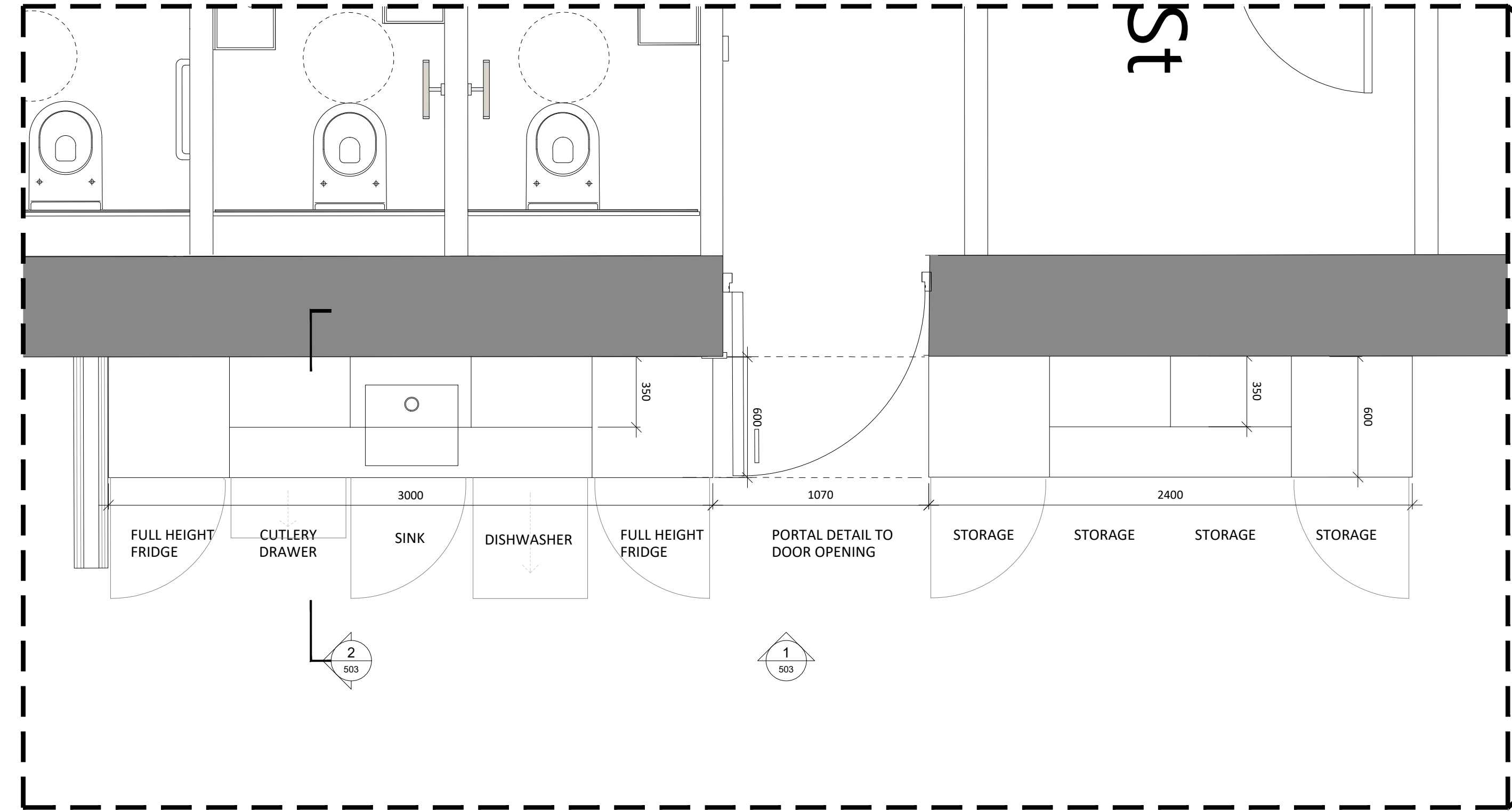
00 THIRD KITCHEN PROPOSED 503 SCALE - 1:20 @ A1 KITCHEN
