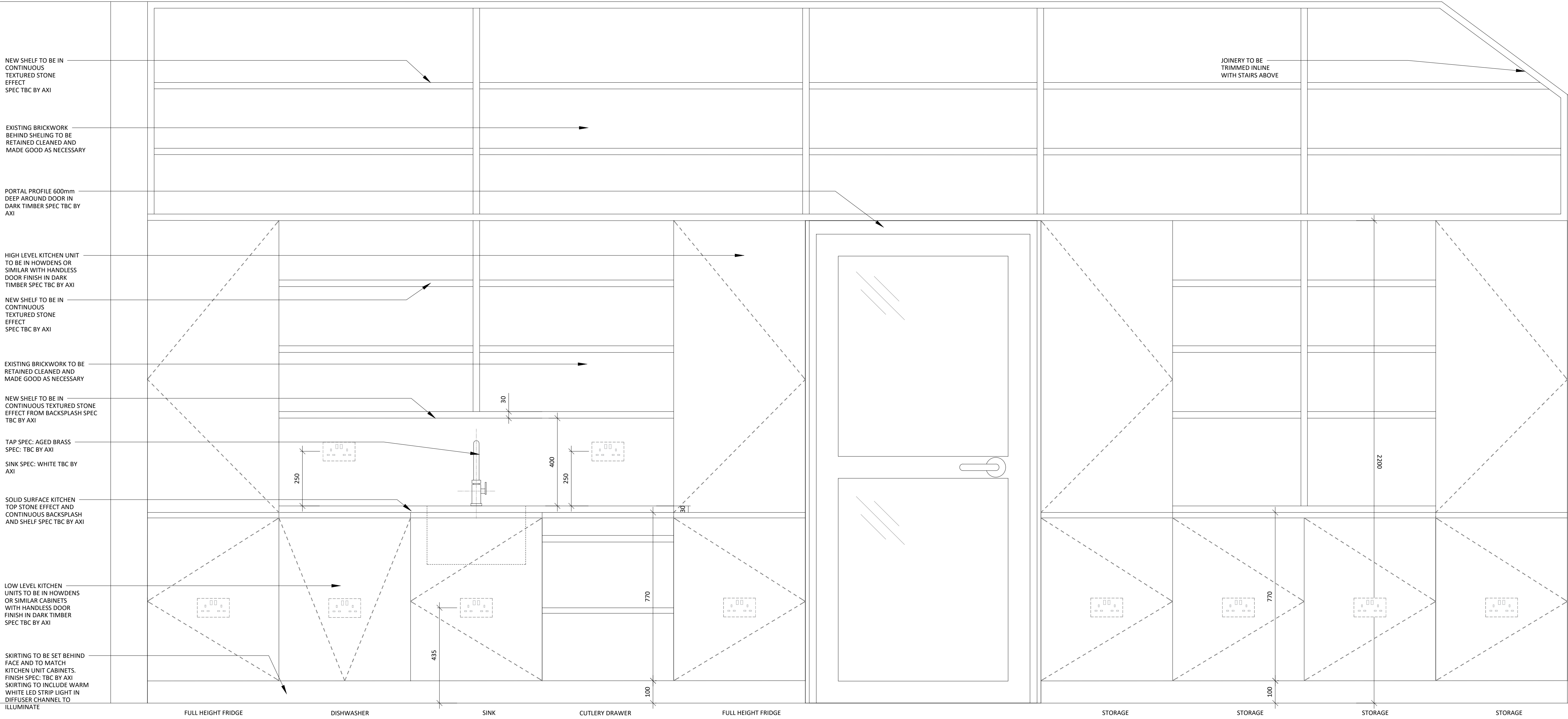
01 PROPOSED KITCHENETTE ELEVATION 503 SCALE - 1:10 @ A1 ELEVATION
