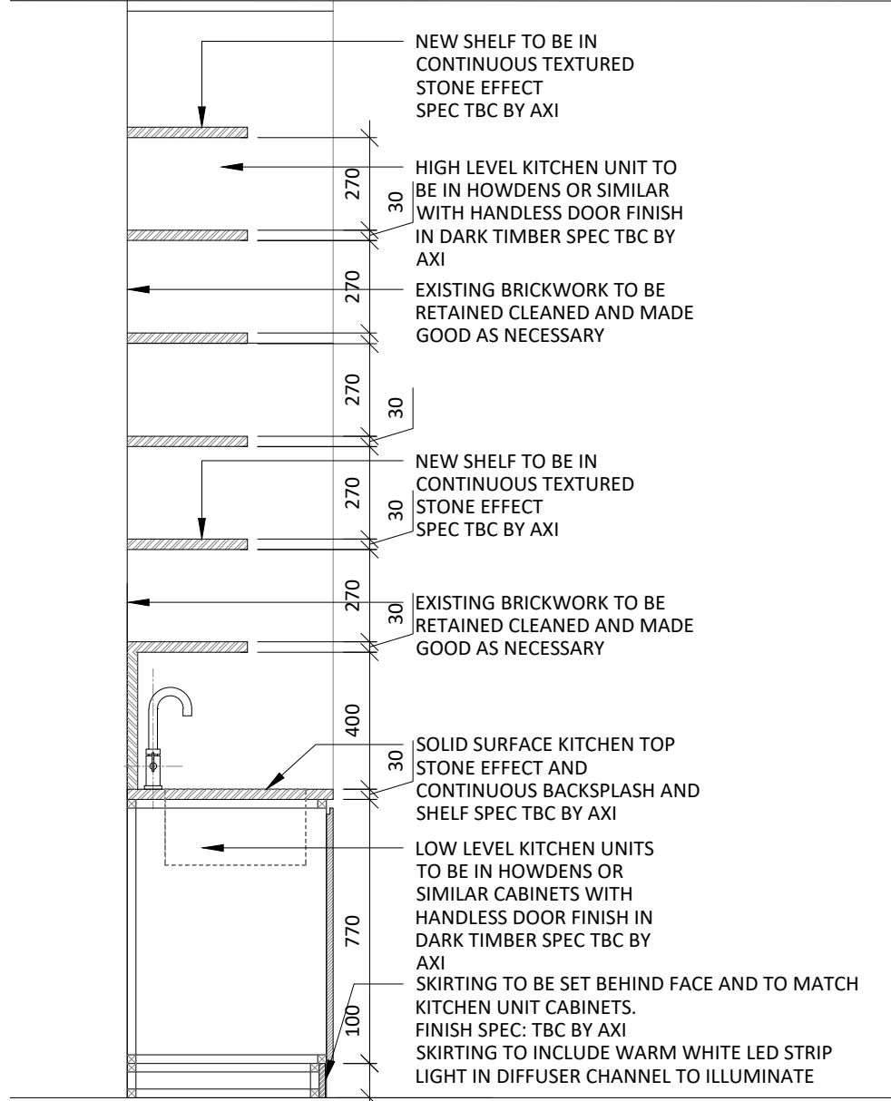
02 PROPOSED KITCHEN SECTION 503 SCALE - 1:20 @ A1 SECTION
