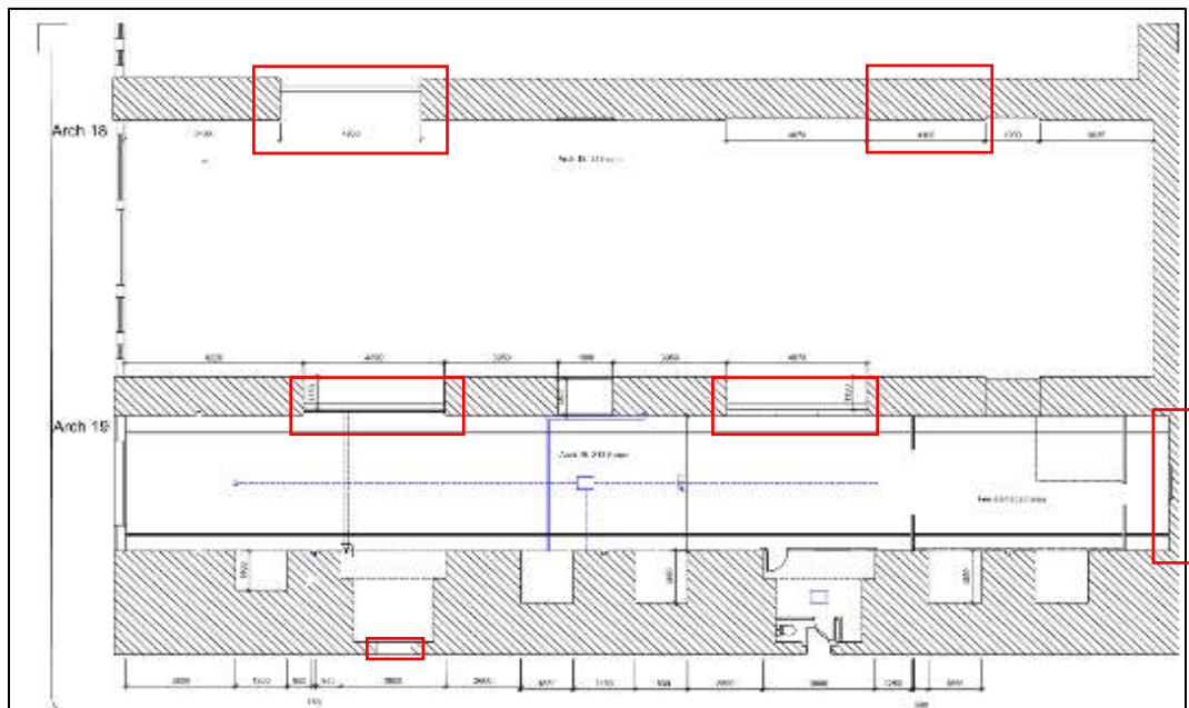
Figure 21: Ground floor plan of the existing Site. 2019. Areas which have now been blocked (since 1899) are shown on the plan in red. Source: Up North Architects.
