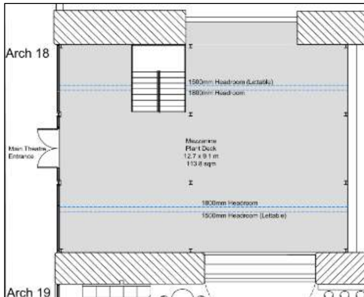
Figure 35: Proposed plans for interior (Mezzanine level). Plan forms the basis of discussion for the physical impact assessment below. Source: Up North Architects.
