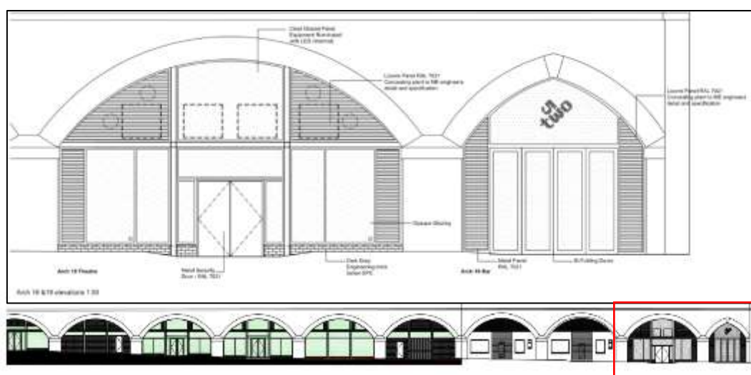
Figure 33: Proposed plans for principal elevation fronting onto Watson Street. The Site is shown within the context of other developments along Watson Street, of similar design/fittings. Source: Up North Architects.
