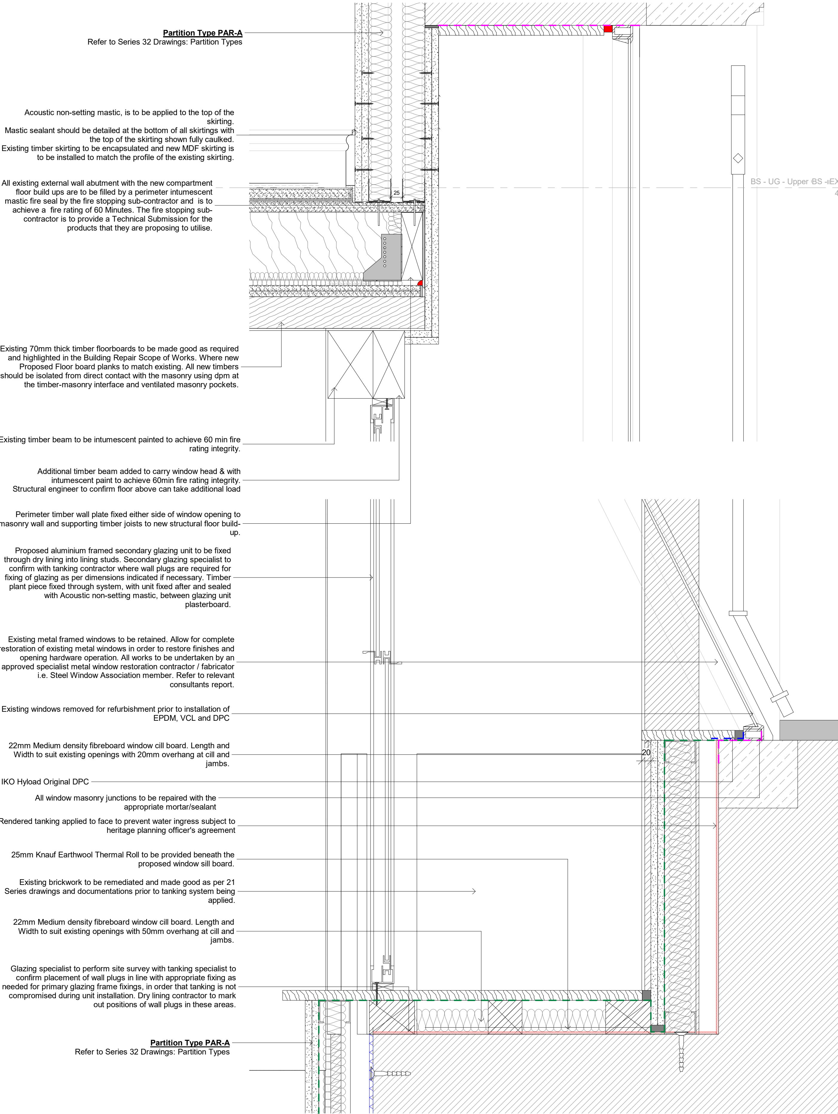
1 | SECTION DETAIL 1:5
