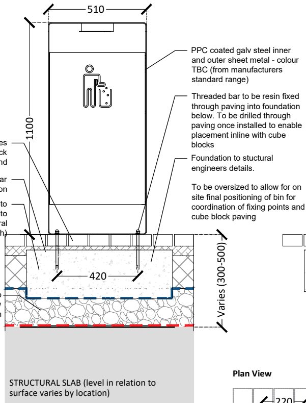
F8 Front Elevation
