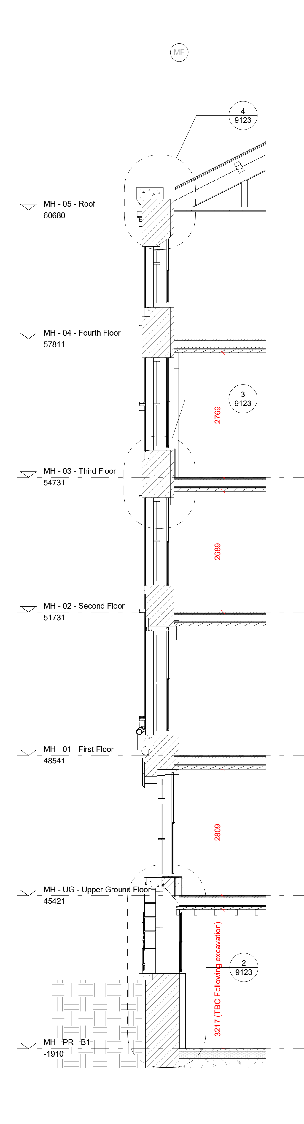
1 | EX WALLS SECTION DETAILS - BLOOM STREET 1 : 50
