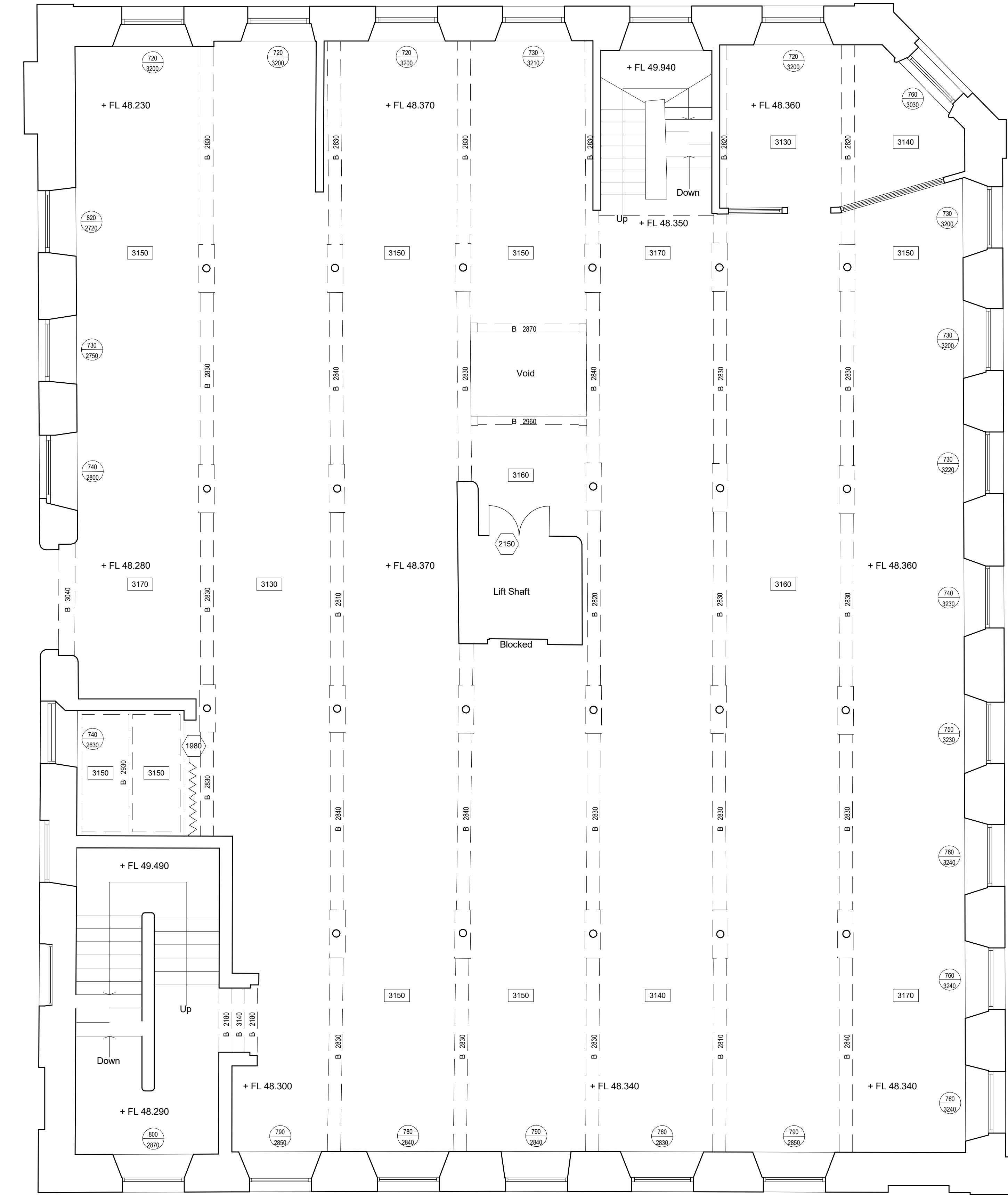
1 | First floor - existing. SCALE 1 : 50 @A1
