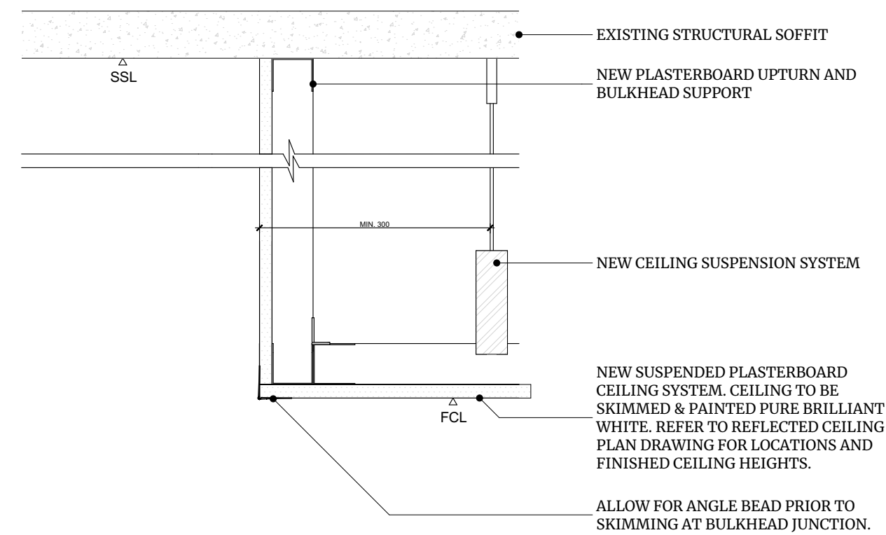
PLASTERBOARD BULKHEAD
