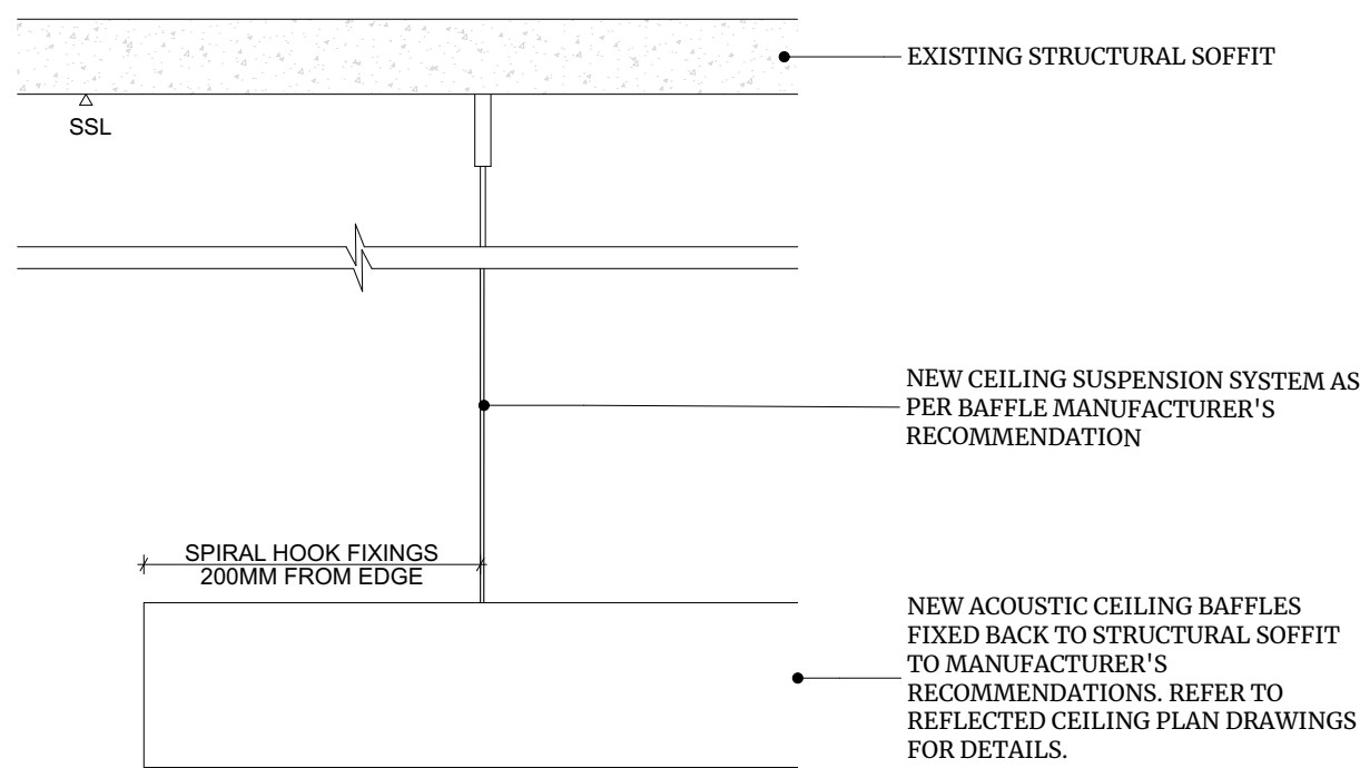
ACOUSTIC BAFFLES TO SOFFIT JUNCTION
