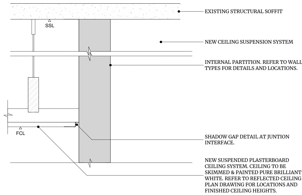
PLASTERBOARD CEILING TO PARTITION JUNCTION
