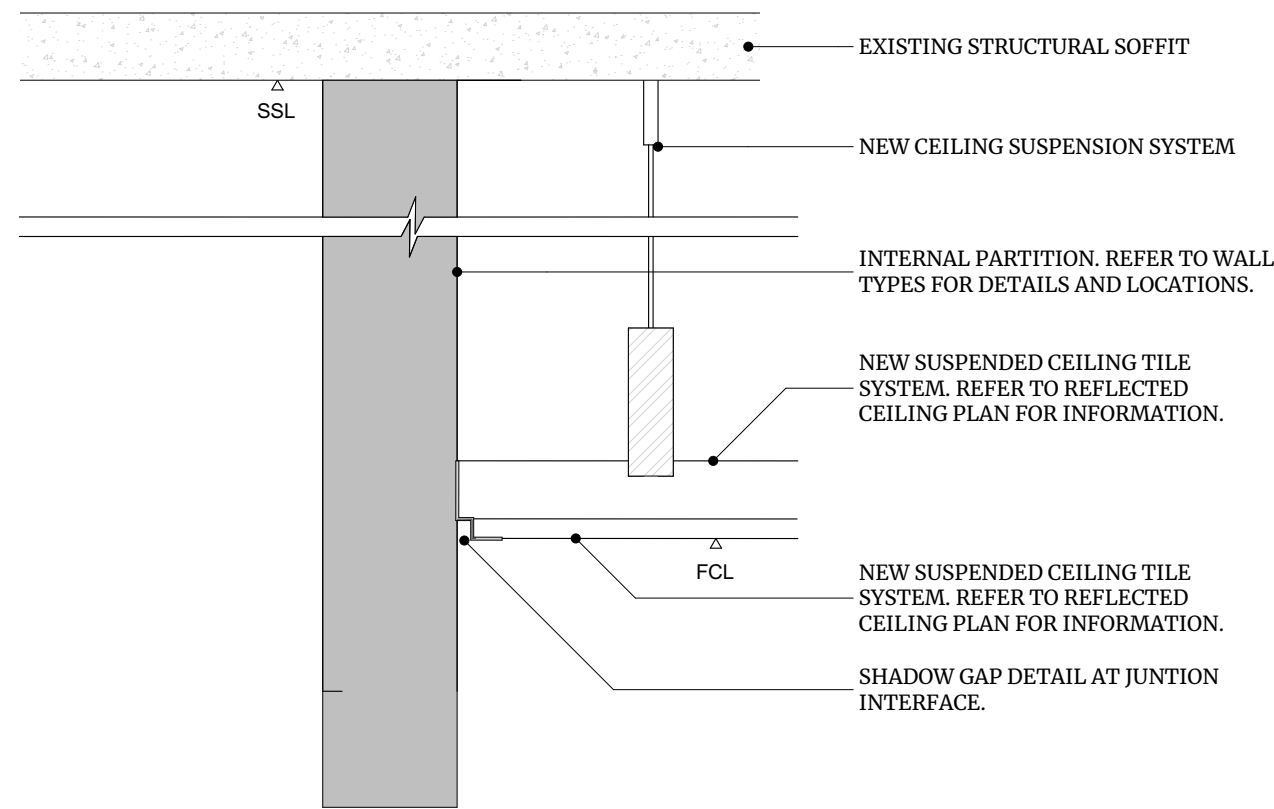
CEILING TILES TO PARTITION JUNCTION
