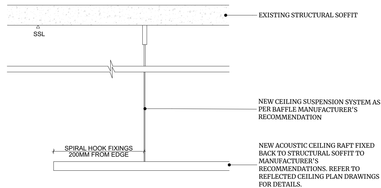
ACOUSTIC RAFTS TO SOFFIT JUNCTION
