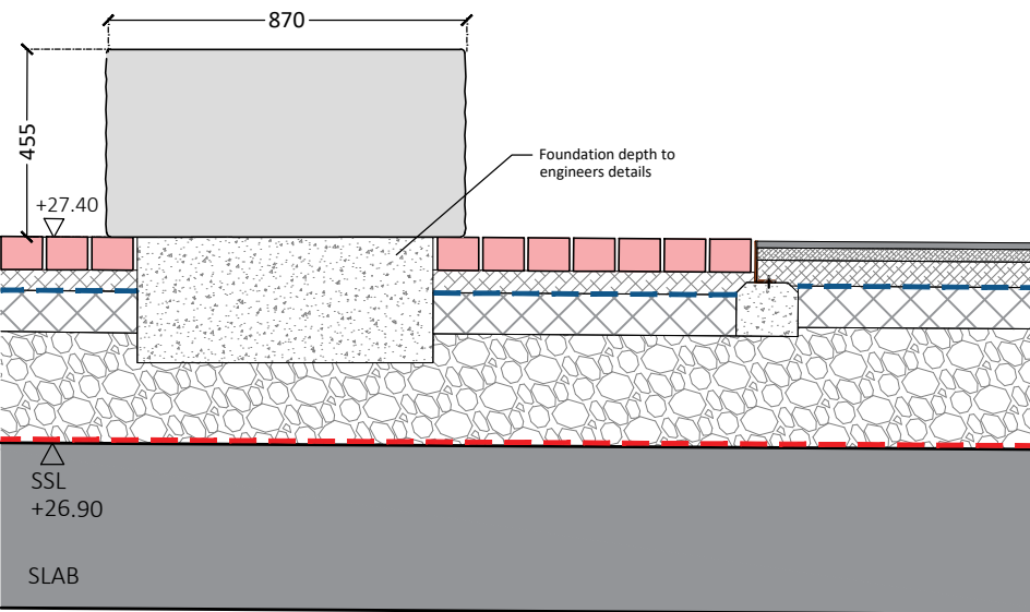
SECTION AA 1:20
