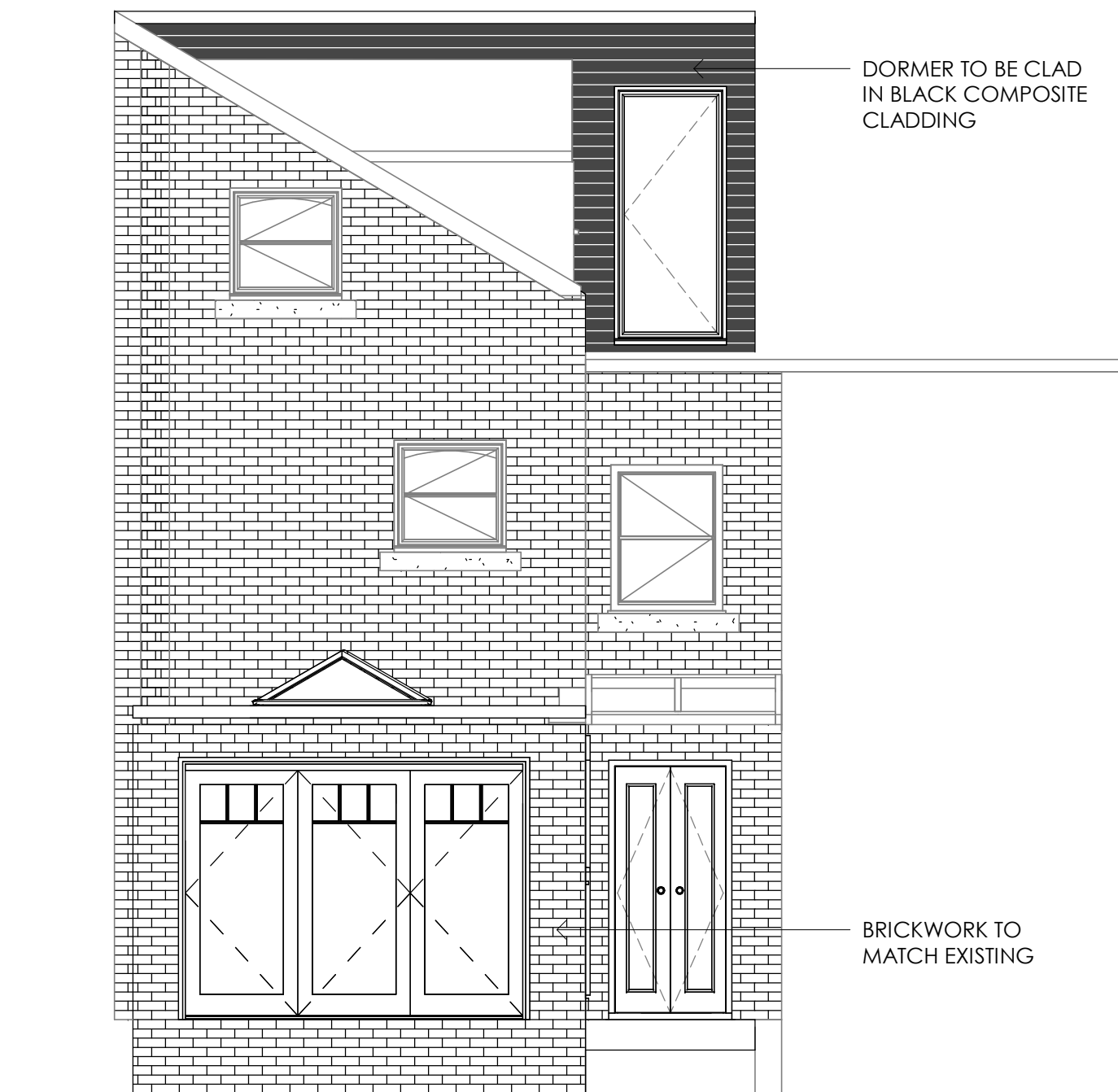
2 PROPOSED SIDE ELEVATION 2 1 : 50
