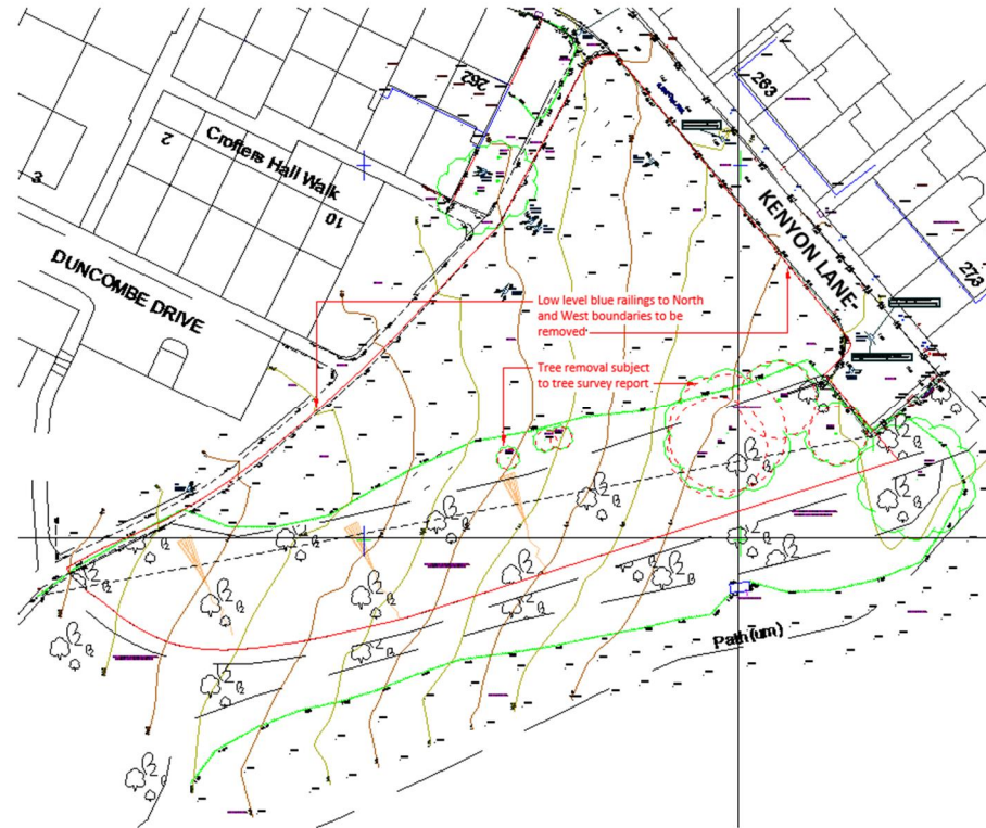
Site Clearance Plan
