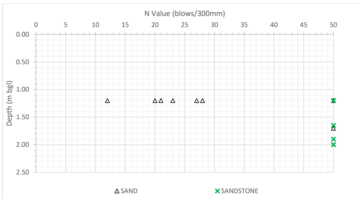
Figure 4: SPT Results
