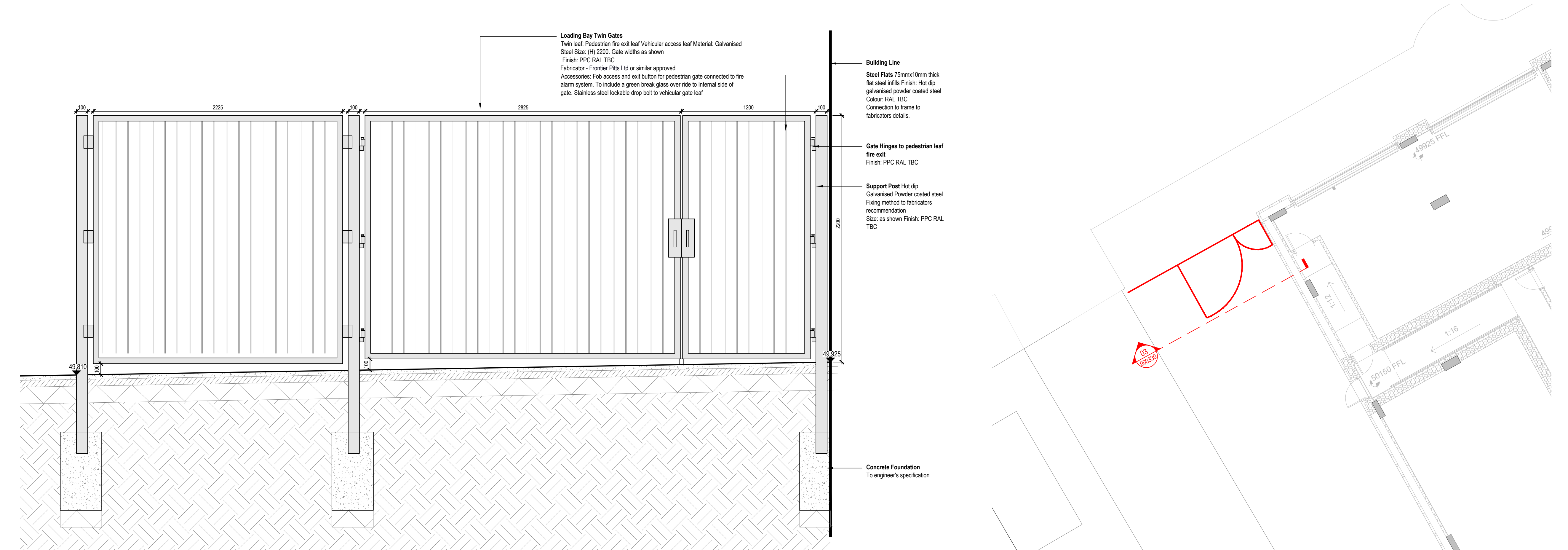
03 900330 B2 - Bespoke Steel Maintenance Access Gate Scale 1: 20 @A1
