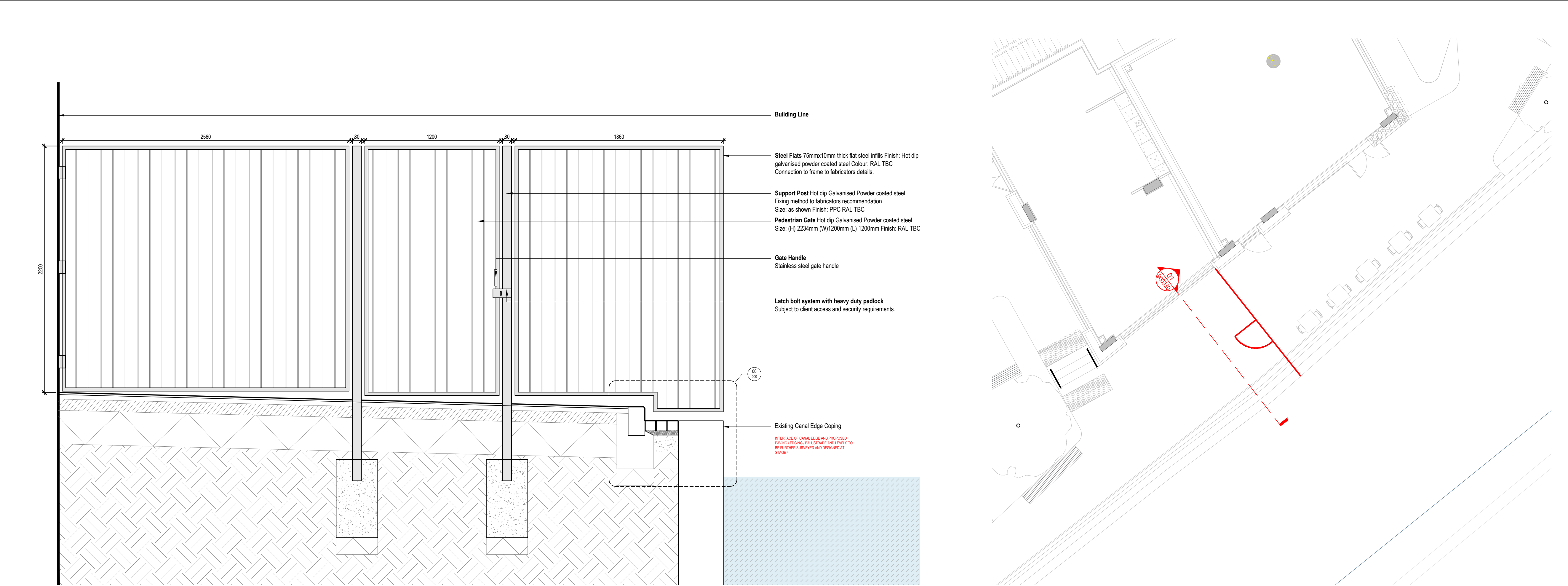
01 900330 B1 - Steel Fencing and Pedestrian Access Gate Scale 1: 20 @A1
