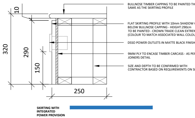
02 POWER SKIRTING PROFILE DETAIL 409 SCALE - 1:10 @ A1
