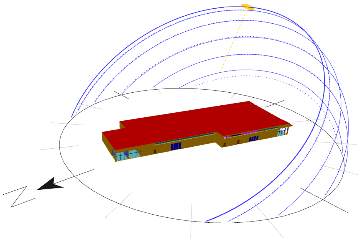
Figure 9 - Orientation & Sun Path Image
