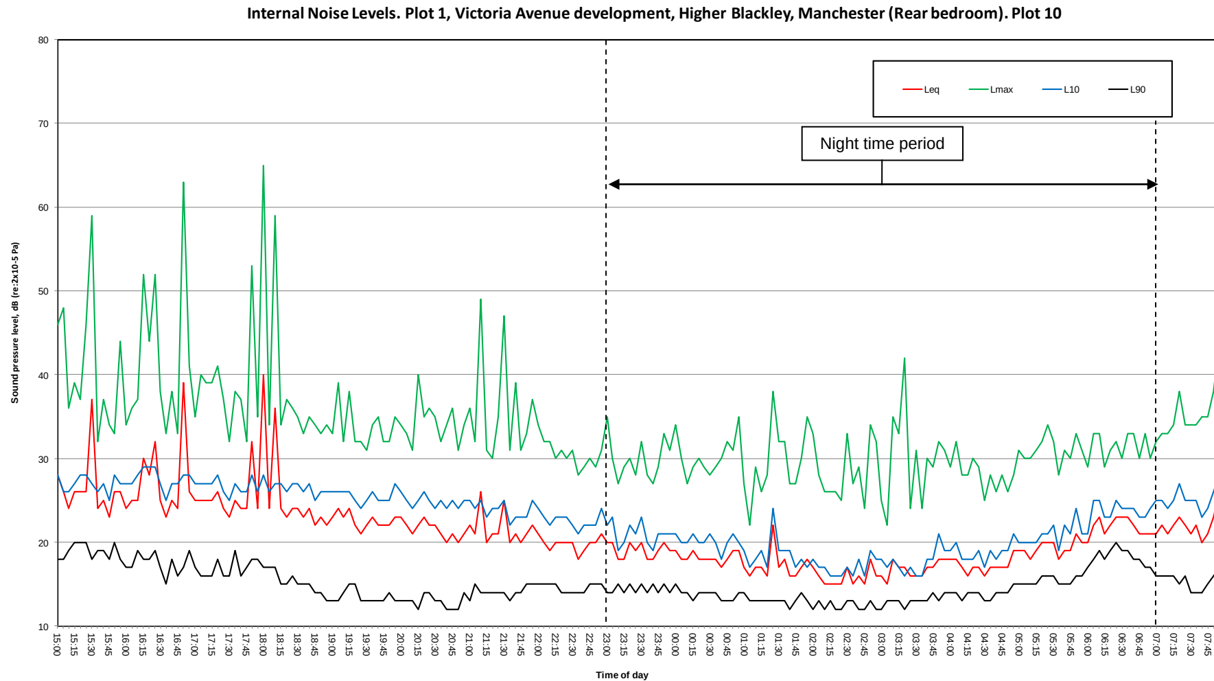
Graph 2. Standardised sound level summary, rear bedroom, plot 10
