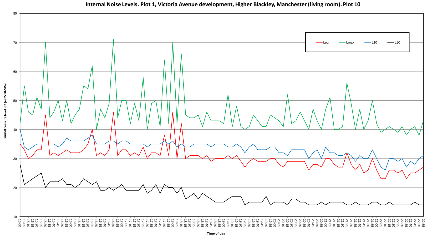
Graph 3. Standardised sound level summary, living room, plot 10
