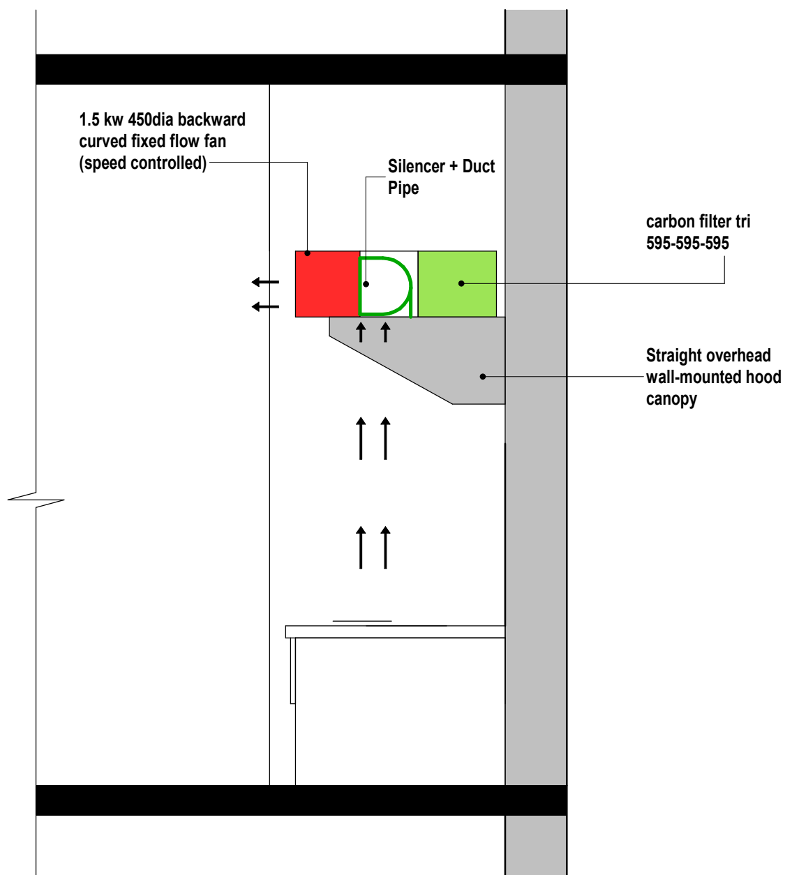
Proposed Section 2 1 : 30
