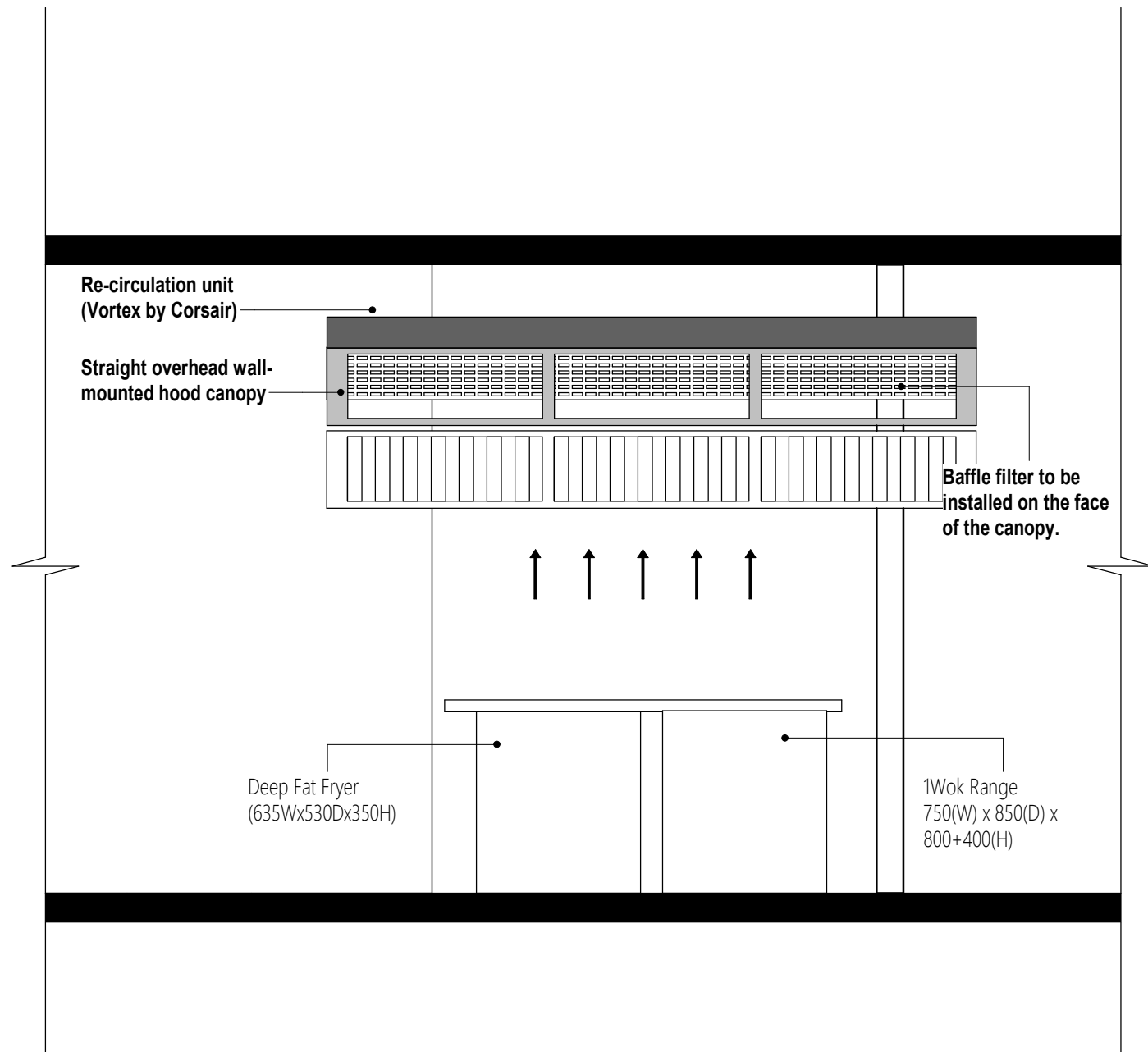
Proposed Section 1 1 : 30
