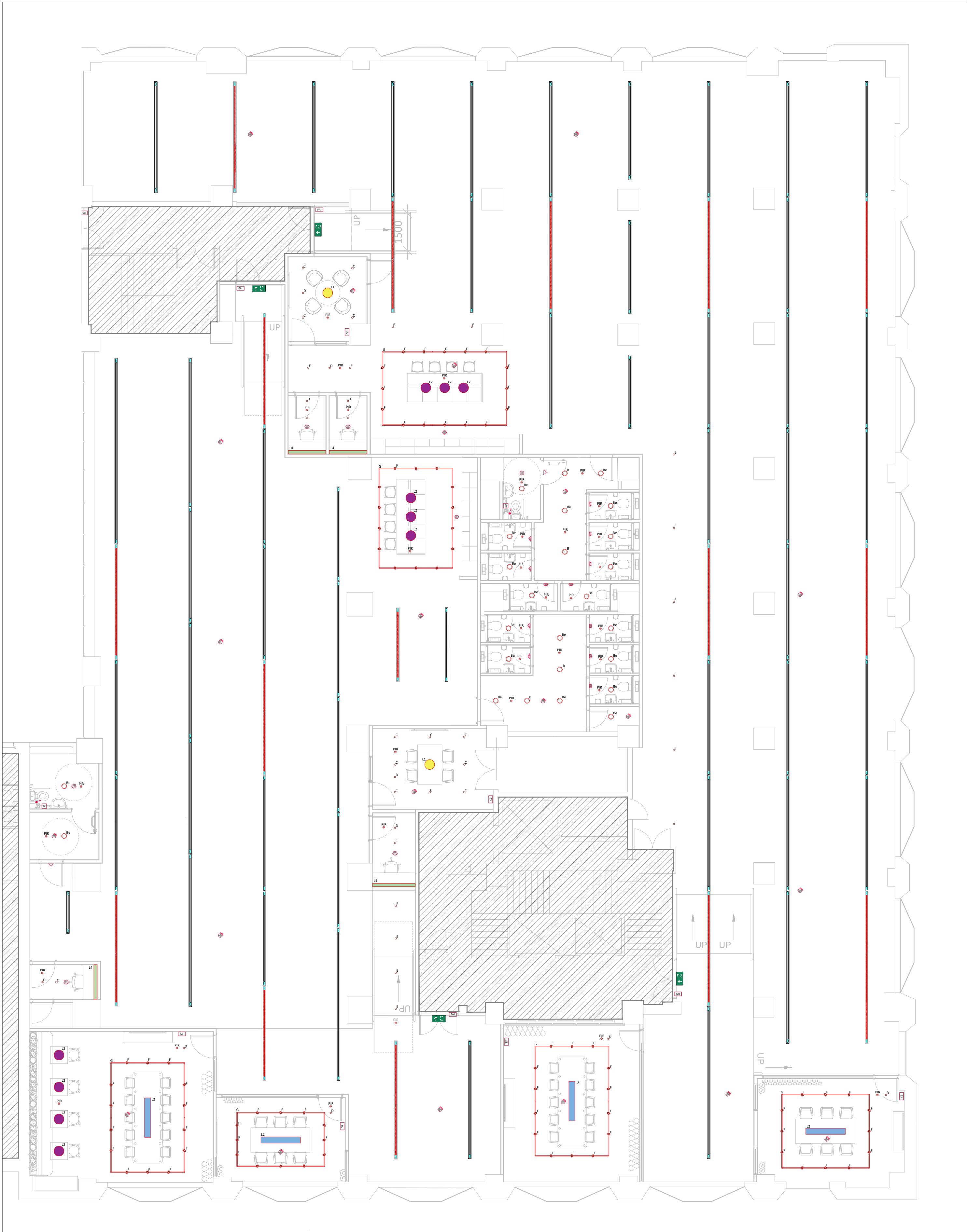
Lee House | Third Floor Lighting & Fire Alarm
