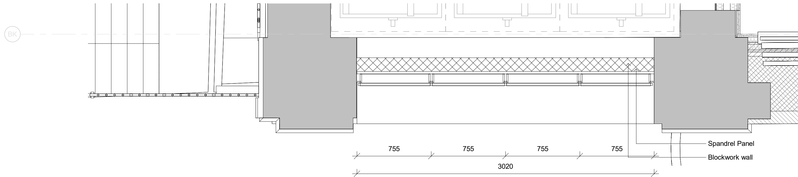
2 | Bin Store Curtain Walling - Plan Copy 1
