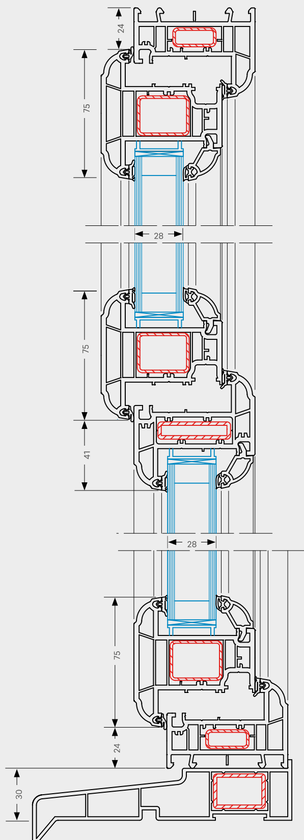
Below: Vertical Section (Sculptured)
