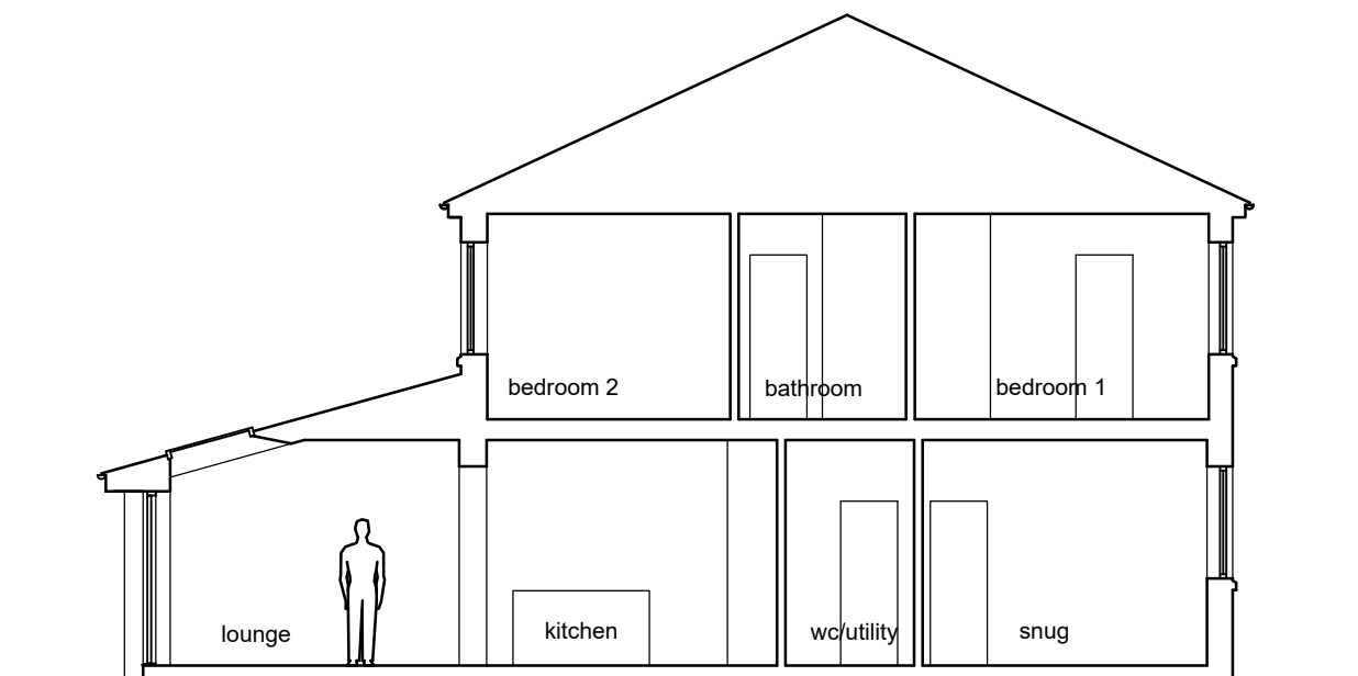
PROPOSED SECTION
