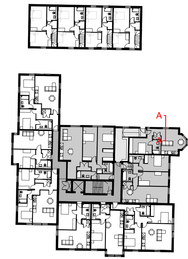
KEY PLAN - UPPER GROUND FLOOR 1:400@A1
