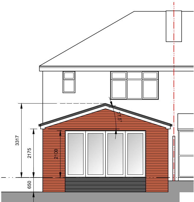
South West Facing Rear Elevation
