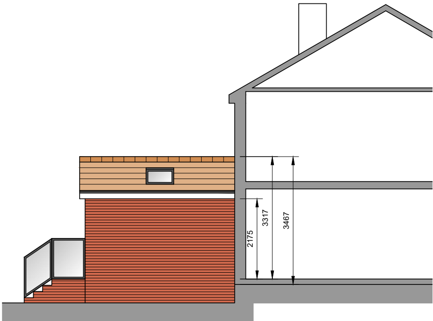
South East Facing Side Elevational Section
